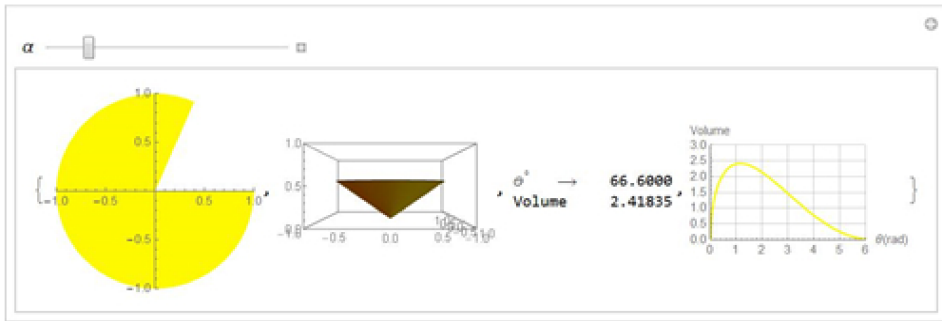
Figure 3. Output of the Mathematica code embodying all the needed information.
