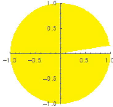
Figure 1. A unit disk with a cut out circular sector.
