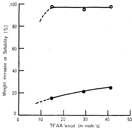
Fig. 3. Effect of ratio of TFAA (or \beta -MC) to wood on reactivity (O) and solubility (●).
