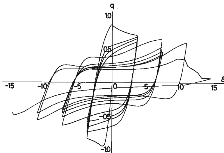
Fig. 19. q - \delta relation of DIC 2.
