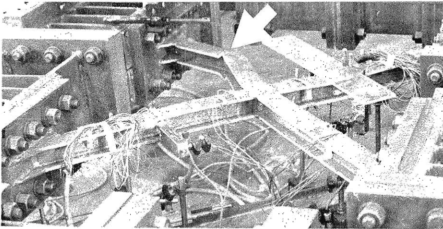
Photo 4. (a) Concentration of bending deformation.
