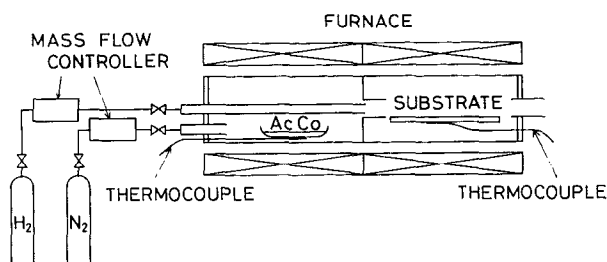
FIG. 1. Schematic representation of experimental equipment.
