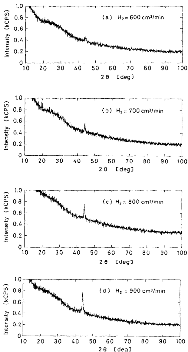
FIG. 4. X-ray diffraction pattern of \sim 100 -nm-thick cobalt film for H_2 flow rate: (a) 600 cm 3 /min, (b) 700 cm 3 /min, (c) 800 cm 3 /min, and (d) 900 cm 3 /min.
