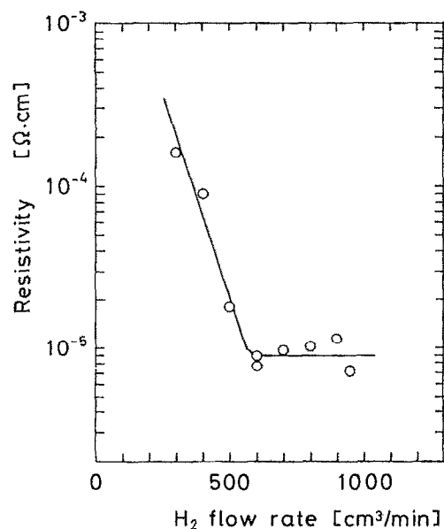
FIG. 3. Resistivity of cobalt film as a function of H_2 flow rate.
