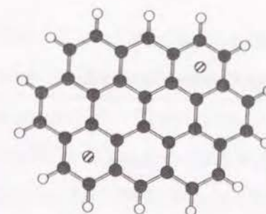
(a) \text{Li}_2 \Delta H_f = 6.944 \text{ eV} charge 1.00
