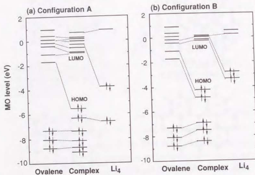
Figure 7. Calculated MO diagram of the four Li adsorbed ovalene systems with configurations (a)A and (b)B.
