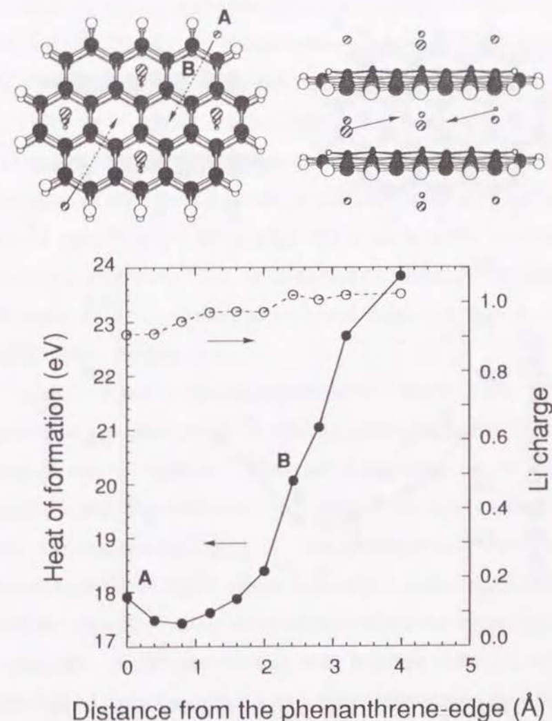
Figure 4. Comparison of the energy profiles of (a)intercalation and (b)adsorption. In the 12 Li doped systems (4 and 8 Li atoms intercalate and adsorb, respectively), extra two Li atoms (a)intercalate and (b)adsorb as indicated by the arrow. Closed and open circles show the heat of formation and charge of the extra Li, respectively.
