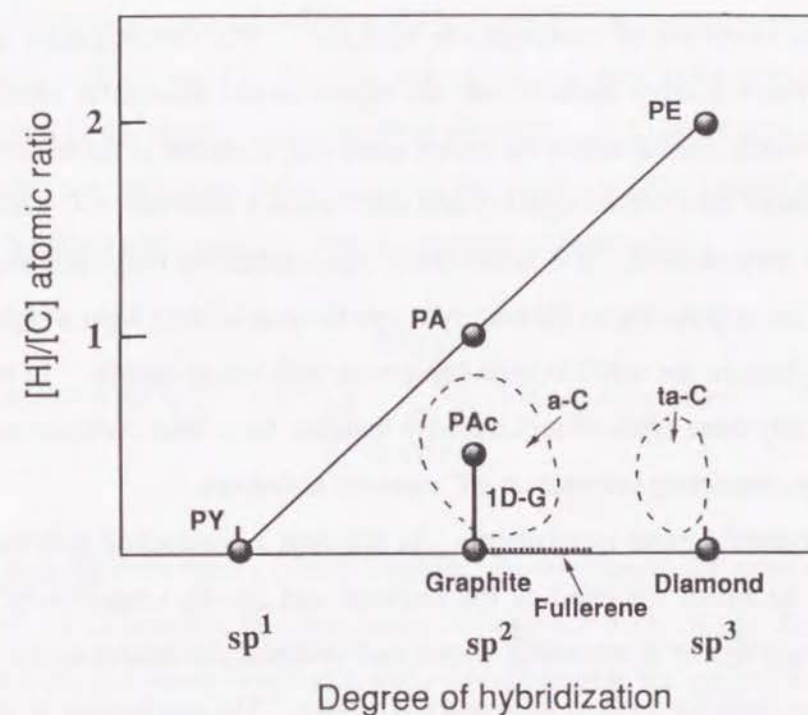
Figure 1. A "phase" diagram including carbon materials and organic polymers. PY, PA, PE, PAc, 1D-G, a-C and ta-C represent polyynes, polyacetylene, polyethylene, polyacene, one-dimensional graphite family, the amorphous carbon having sp^2 -hybridized carbon atoms, and the tetrahedrally bonded amorphous carbon with sp^3 -hybridization, respectively.
