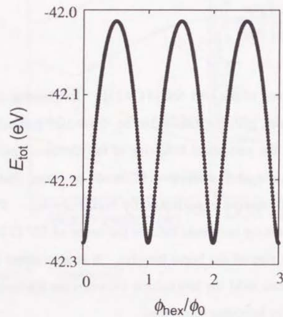
Figure 4. Total electronic energy per cell vs. \phi_{\text{hex}}/\phi_0 .
