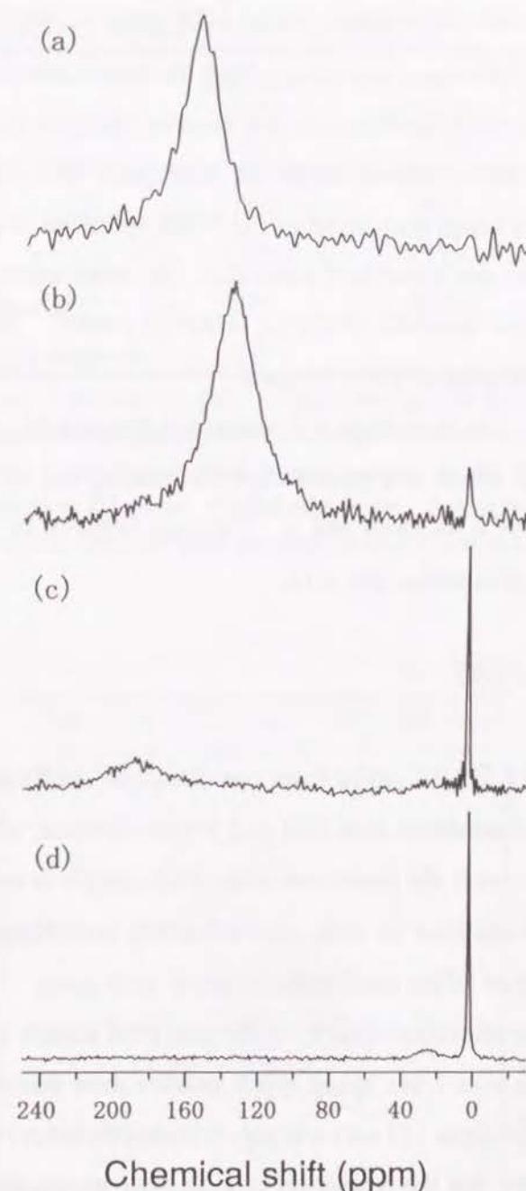
Figure 1. 129 Xe NMR spectra under 5 atm of Xe gas of (a) the pure PAS, (b) the PAS electrode kneaded with PTFE binder, (c) the dipped PAS electrode impregnated into the 1 M LiPF 6 dissolved PC electrolyte solution, and (d) the 5%-Li-doped PAS electrode.
