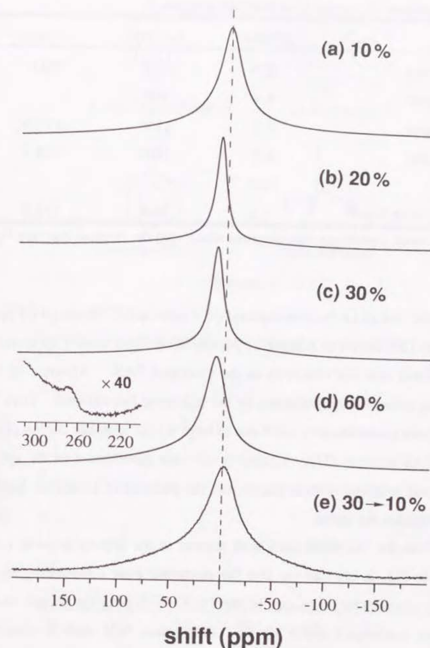
Figure 1. ^7\text{Li} NMR spectra of (a)10 %-, (b)20 %-, (c)30 %-, (d)60 %-doped, and (e)30 \rightarrow 10 %-undoped samples measured at room temperature. The 1 M LiCl solution was employed as an external standard.
