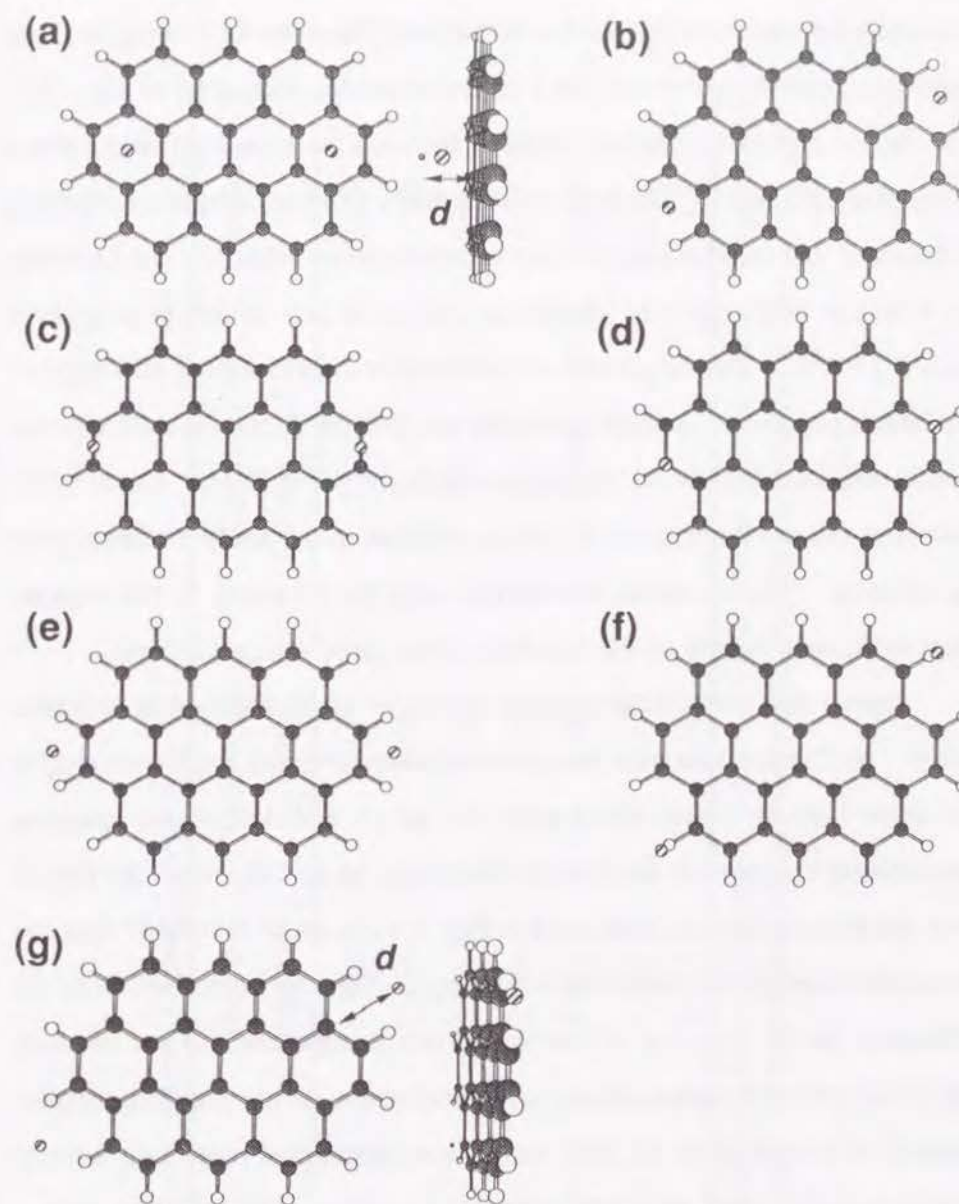
Figure 1. Configurations of two-Li-doped ovalene systems. The Li atoms are located over (a) center of benzene ring (ring-over site), (b) acene-edge (acene-edge site), (c) C—C bond (bond-over site), (d) C atom (atom-over site), (e) phenanthrene-edge (phenanthrene-edge site), and (f) the line on the C—H bond (C—H bond-over site). The vertical distance, d , between the Li and the ovalene sheet was optimized. In configuration (g), the Li atoms are located on the same plane with ovalene and the distance between the edge carbon was optimized.
