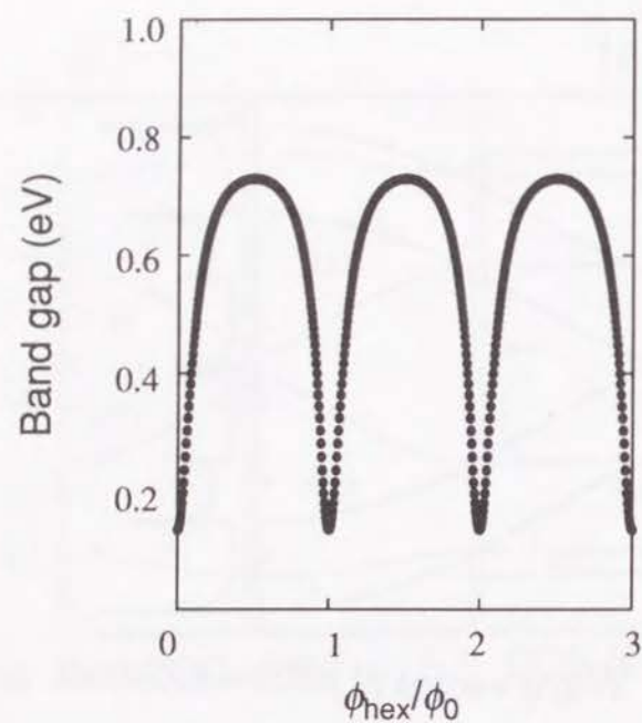
Figure 3. Change of the band gap with respect to the magnetic field represented by \phi_{\text{hex}}/\phi_0 .
