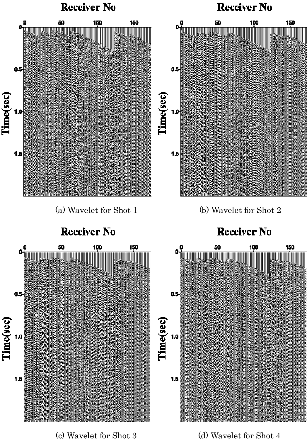
Fig 4-5 Common shot records after preprocessing
