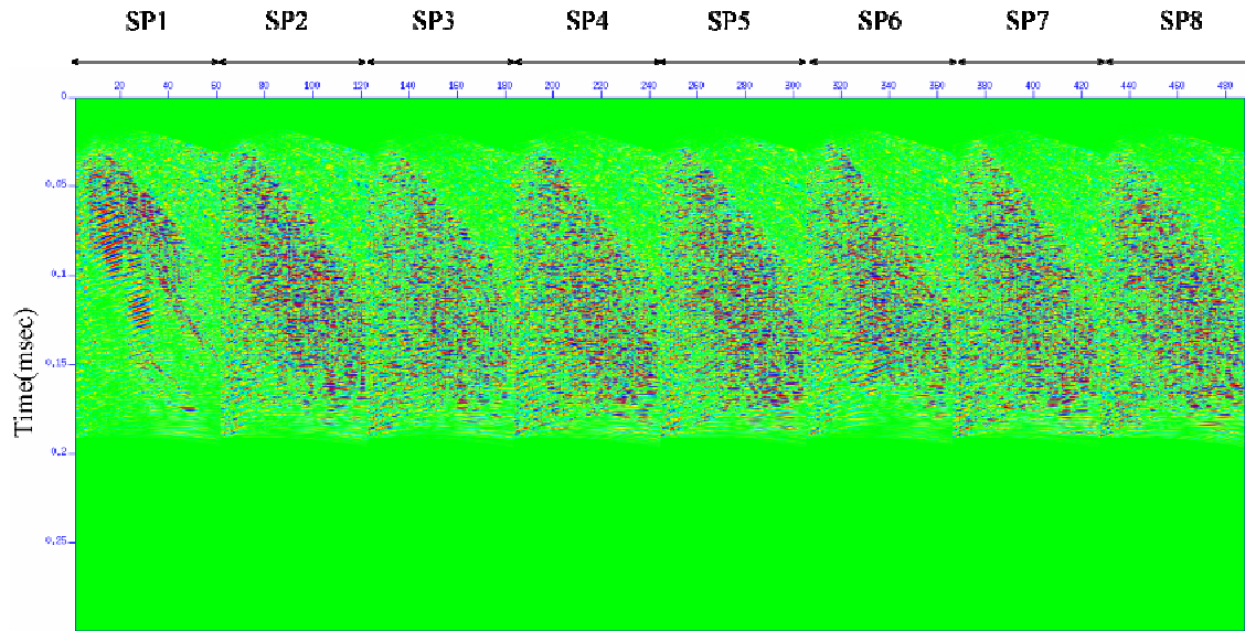
Fig 4-27 Inverse IP transform results for the data shown in Fig 4-25
