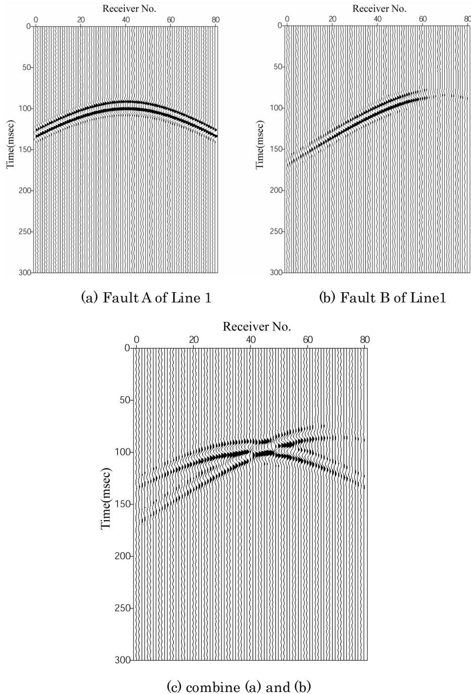
Fig 3-27 Generalized inverse IP transform results for Line 1
