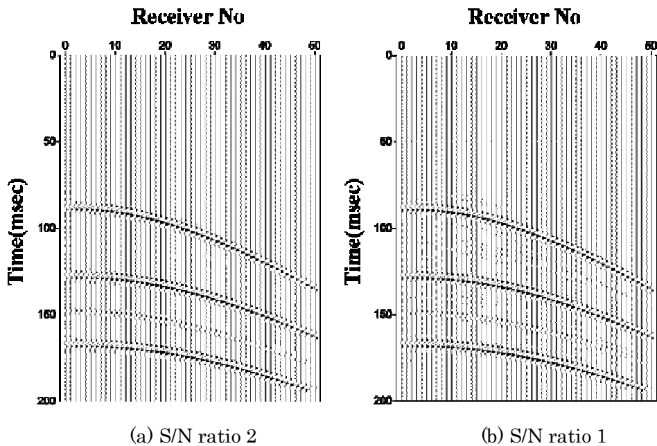
Fig 3-9 Inverse IP transform results of multiples
