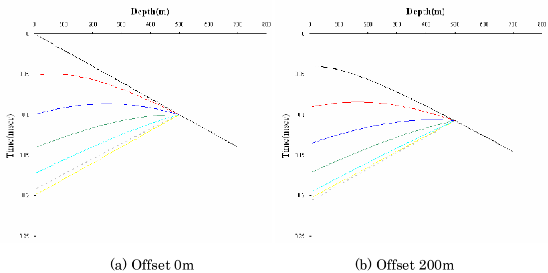
Fig 3-20 Analytic travel time curve
