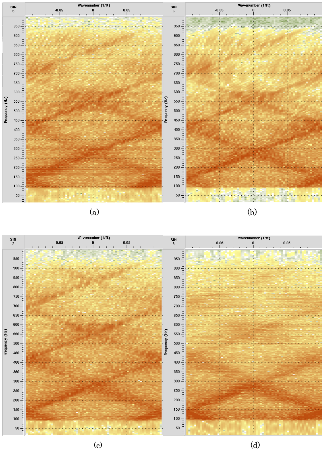
Fig 4-21 F-K analysis results for the SP5 (a), SP6(b), SP7(c) and SP8(d)
