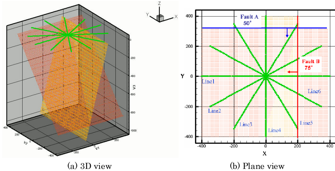
Fig 3-21 3-D two faults model
