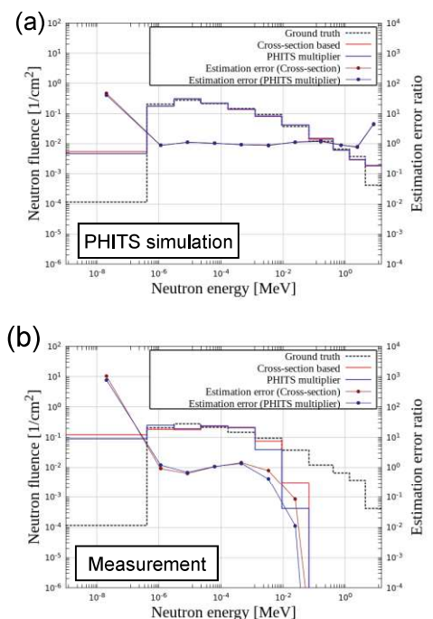
Fig. 2. Estimated neutron energy spectrum by SOF detector.
