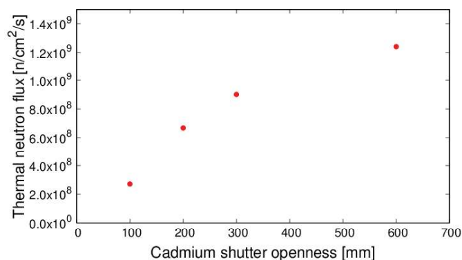
Fig. 1. Relationship of the thermal neutron flux and the cadmium shutter openness.
