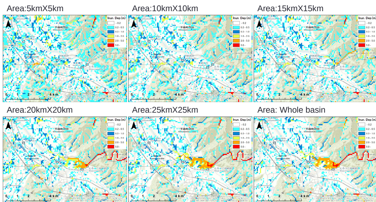
Fig. 11 The distribution of maximum inundation depth in the scenario of the 200-year probability rainfall strength in each rain-area.
