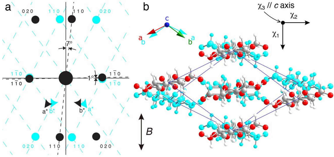
Fig. 7 Twin orientation of (a) reciprocal lattice and (b) real lattice of cellulose II crystals by the static magnetic field. A double-headed arrow indicates the direction of the magnetic field. The [1\ 1\ 0] and [1\ \bar{1}\ 0] directions are tilted by about 7^\circ and 1^\circ from \chi_1 and \chi_2 directions, respectively. The chain axis ( c -axis) direction \parallel \chi_3 is perpendicular to the plane of the paper.
