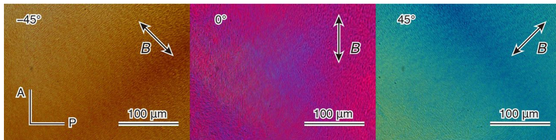
Fig. 5 Cellulose II crystals/PVA films dried under horizontal static magnetic field of 8 T were observed under polarized microscope with color plate. The double-headed arrow indicates direction of the magnetic field. The film was rotated by \pm 45^\circ with respect to the polarizer (P) and analyzer (A).
