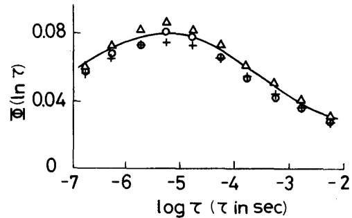
Fig. 1.8. Distribution function of relaxation times at -49^\circ\text{C} for absolutely dried HOONOKI in L direction. ( \gamma = 0.48 , solid line: Eq. (1.15) open circles: Eq. (1.16) triangles: Eq. (1.11) crosses: Eq. (1.13)).
