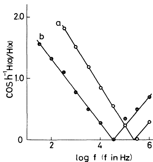
Fig. 1.7 \cosh^{-1}H(0)/H(x) versus \log f curves for absolutely dried HOONOKI in L direction. (a: \gamma=0.55 T=-20^{\circ}\text{C} , b: \gamma=0.48 T=-49^{\circ}\text{C} ).
