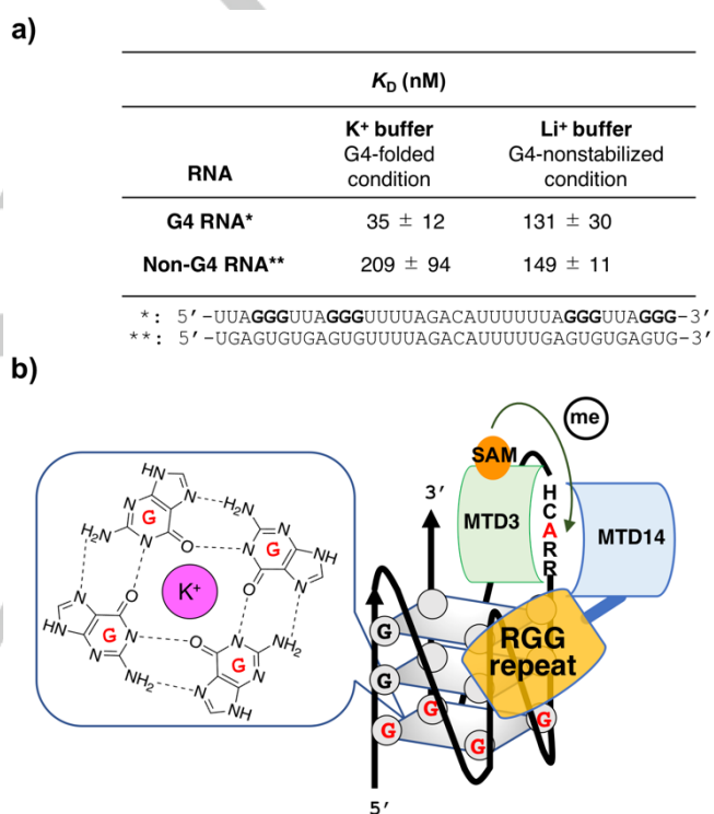
Figure 3. Intrinsic sequence preference of METTL3/METTL14 heterodimer to G4 structure RNA. (a) Dissociation constants of MTD3 and MTD14 heterodimer with the RGG domain [58] . Note that the G4 RNA oligonucleotide forms the G4 structure in K + buffer but not in Li + buffer. (b) Schematic representation of preferential m^6A methylation close to the RNA G4-structure. The inset shows a G-tetrad plane. In G4 structures, multiple G-tetrad planes are stacked and stabilized by K + .
