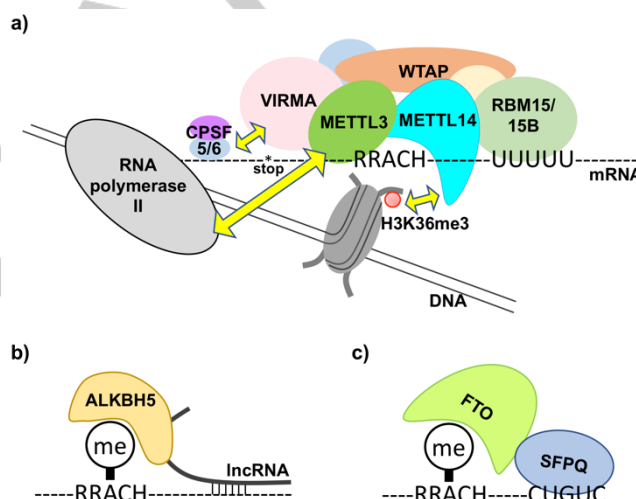
Figure 2. Mediator-guided regulation of m^6A demethylation and methylation. (a) METTL3/METTL14 heterodimer interacts with multiple proteins including RBM15/15B, which binds to U-rich sequences, and VIRMA, which interacts with polyadenylation cleavage factors CPSF5 and CPSF6, resulting in methylation close to the U-rich sequences and close to the 3' untranslated region (UTR) and stop codon. Direct interaction of the METTL3/METTL14 heterodimer with RNA polymerase II along with H3K36me3 histone modification comprise the transcription-coupled m^6A RNA methylation model. (b) ALKBH5 interacts with lncRNAs to demethylate m^6A near lncRNA-binding sequences. (c) FTO interacts with SFPQ, an RNA-binding protein targeting CUGUC sequences, and demethylates bases close to its binding sequences.
