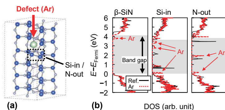
Fig. 1(a) A starting structure of SiN with Ar interstitial, (b) DOS of various SiN structures before and after Ar insertion.
