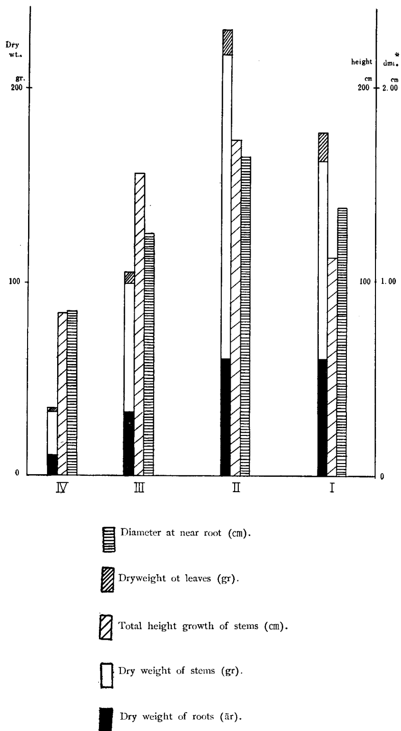
Fig. 1 The variations of dry weight, diameter at near root and height of the stems by the increasing of light intensity.
