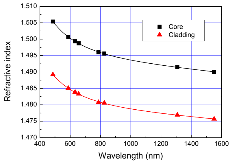
Fig. 9. Refractive indices of core and cladding glasses.
