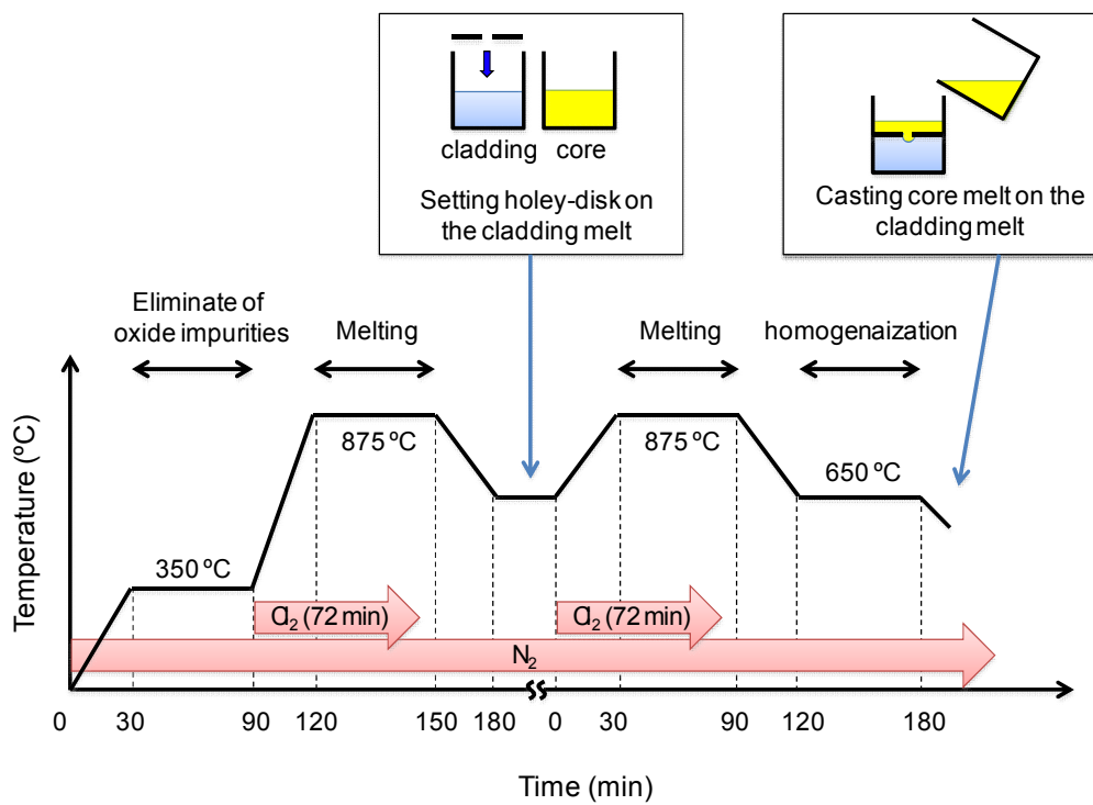
Fig.2. Heating profile for core and cladding glass
