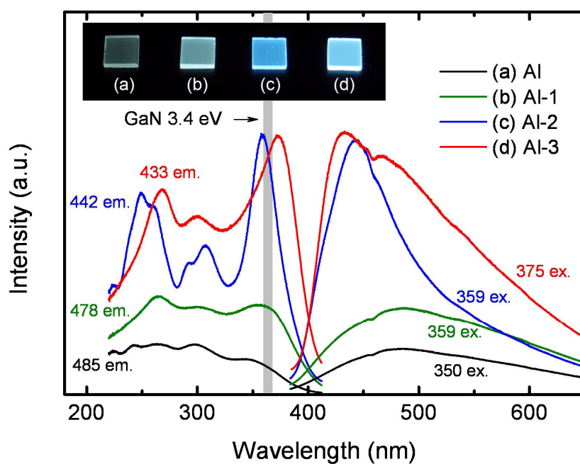
Fig. 7. Excitation and emission spectra for \text{Yb}^{2+}:\text{Al} glasses with added chloride ions. Inset photographs are of samples excited at 365 nm.
