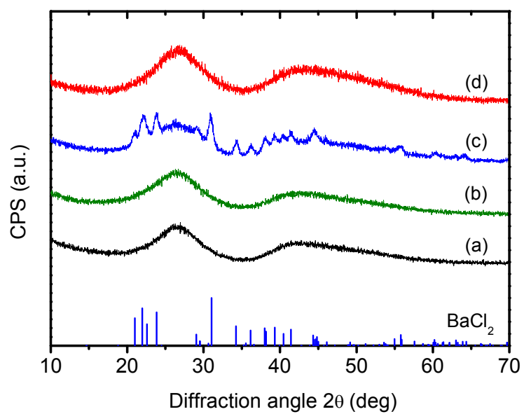
Fig.8. XRD spectra of Yb 2+ :Al glasses melted under a reductive atmosphere.
