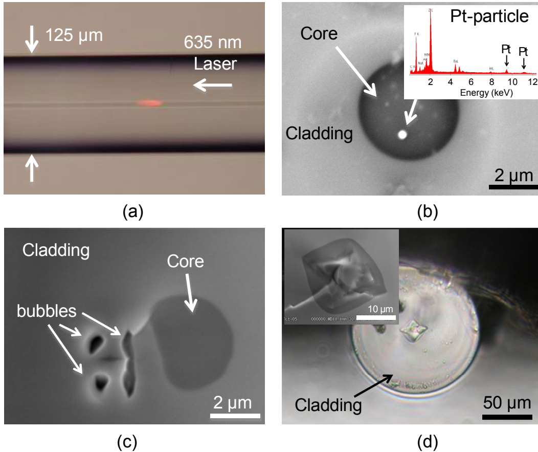
Fig. 12. Defects in fluoride fiber. (a) side view of blight spot while 635 nm laser was coupled into the fiber core. (b) Back scattered electron image of cross section of defect en by cleaving and etching. The composition of white spot was identified Pt. (c) distortion of core shape caused by bubble. (d) Optical microscope image of bright spot exposed by cleaving. The inset figure shows SEM image of the core.
