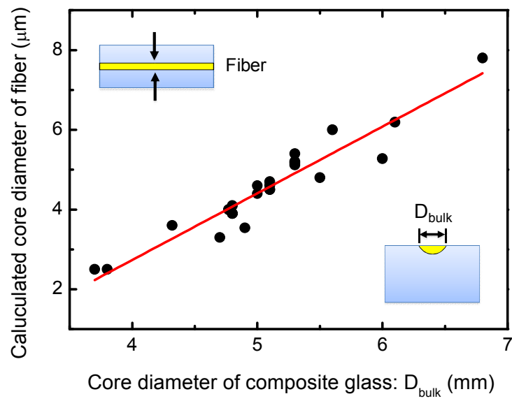
Fig. 8. Relationship between the diameter of composite glass core ( D_{\text{bulk}} ) and the diameter of the core fiber.
