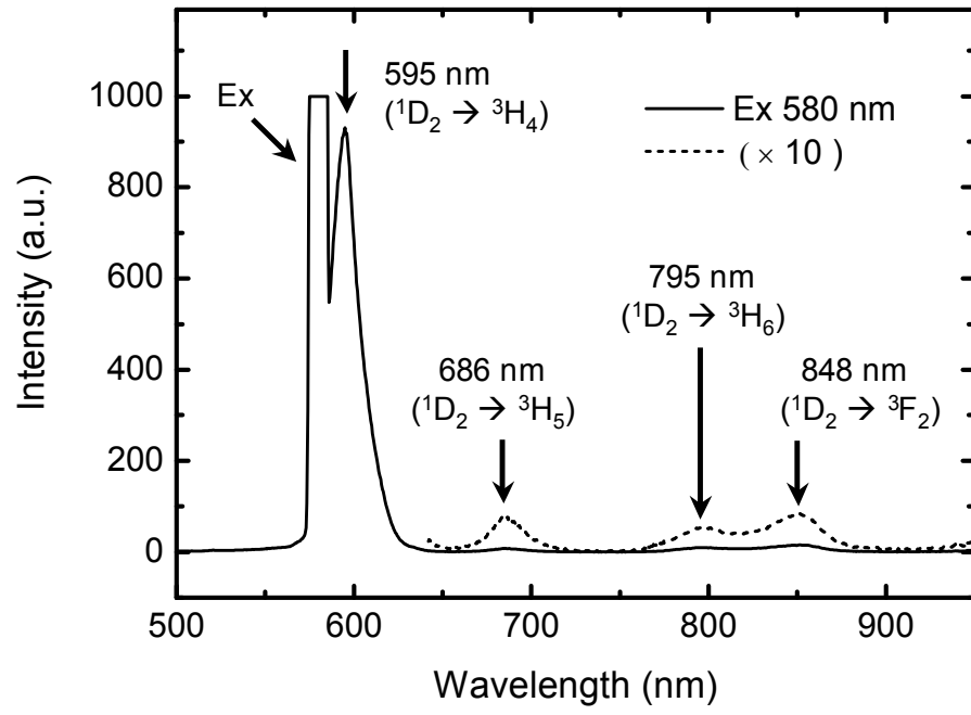
Fig. 6. Fluorescence spectrum of \text{Pr}^{3+}:\text{ZBLAN} under excitation at 580 nm.
