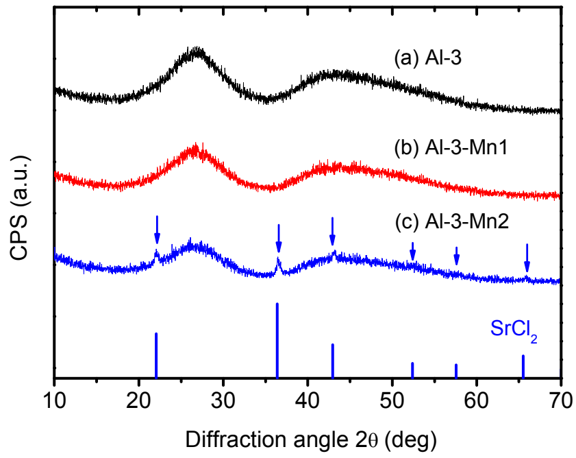
Fig.10. XRD spectra of \text{Mn}^{2+}\text{-Yb}^{2+}\text{:Al} glasses melted under a reductive atmosphere.
