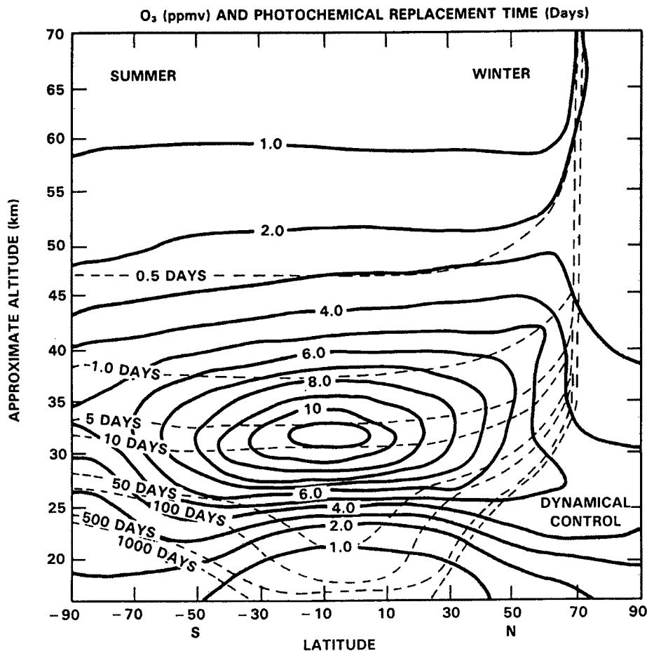
Fig. 6 Computed local photochemical ozone replacement time ( t = local ozone concentration divided by twice the rate of molecular oxygen photolysis) in days (dashed lines) and ozone mixing ratios in ppmv (solid lines) for the end of December 12) .
