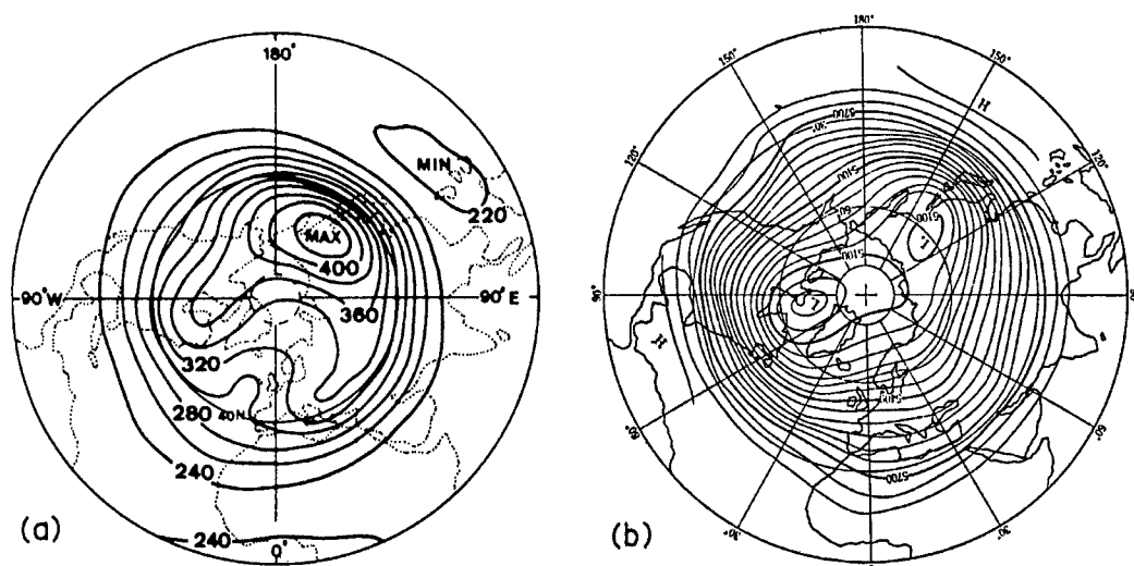
Fig. 4 Monthly average charts for the Northern Hemisphere in January.
