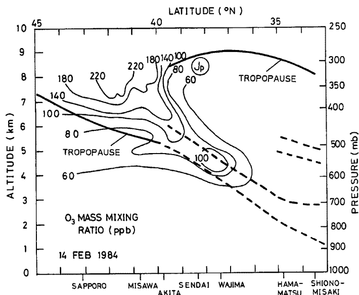
Fig. 14 North-south cross section of ozone through a jet stream. Solid lines show the ozone mass mixing ratio; heavy solid lines, tropopause; heavy broken lines, frontal boundaries; Jp, the axis of polar front jet.
