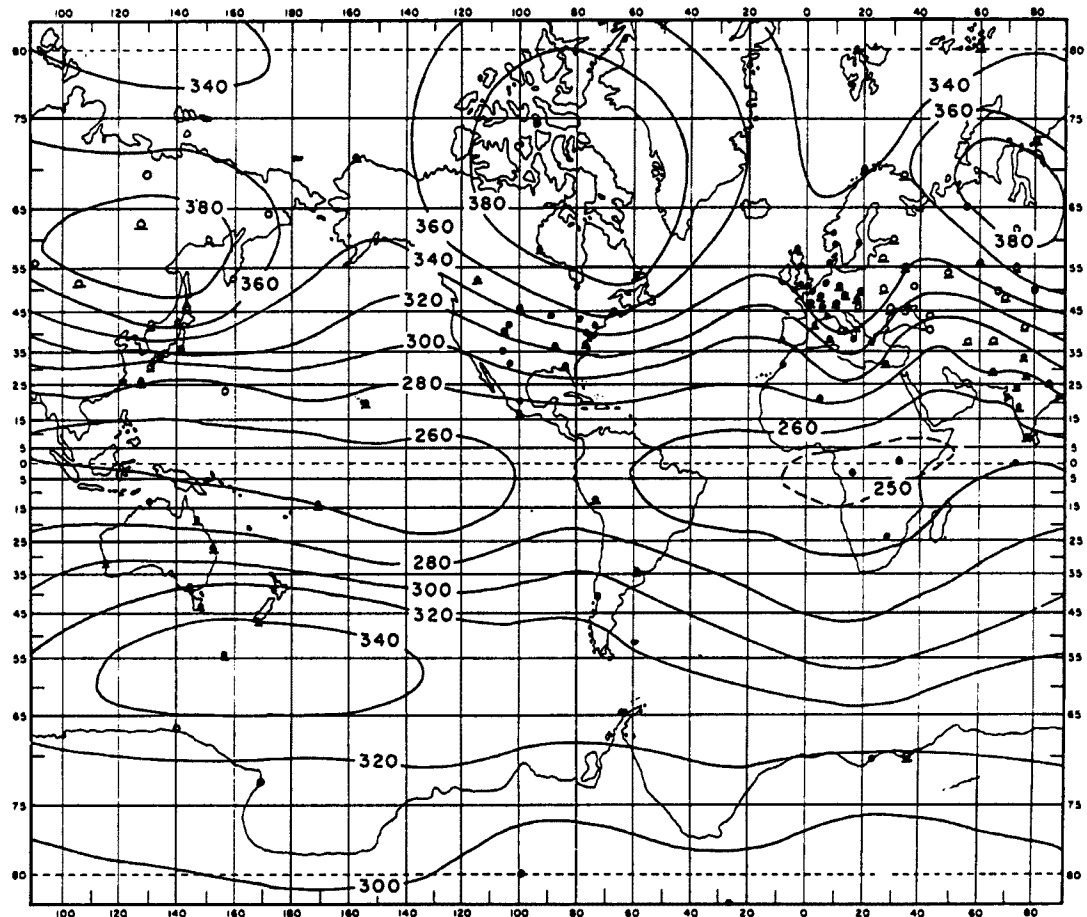
Fig. 3 The average global distribution of total ozone for the period 1958-1977 (Unit: m-atm cm) 11) .
