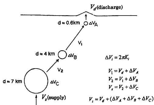
Fig. 14 Schematic diagram for the calculation of magma supply at Mt. Unzen.
