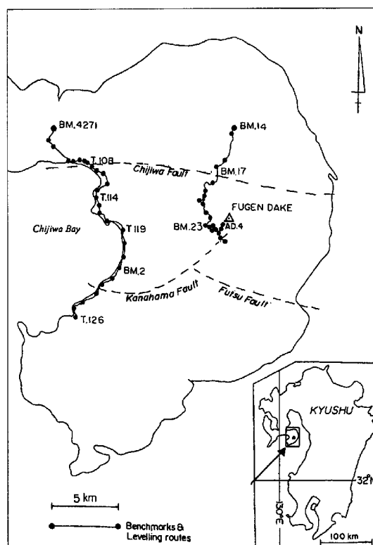
Fig. 1 Location map of leveling routes in the Unzen area, Shimabara Peninsula
