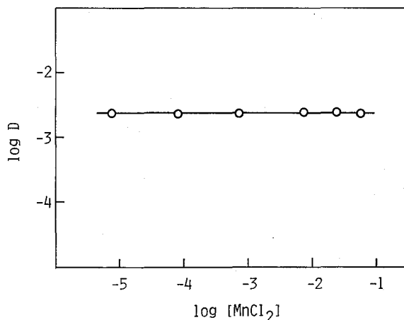
Fig. 4. The distribution ratio of manganese as a function of metal concentration. TOPO: 0.1 M in toluene, \text{HCl} : 1.0 \times 10^{-3}\text{N} , \text{LiCl} : 2.6 \times 10^{-1}\text{M} .
