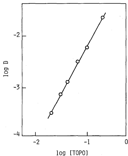
Fig. 3. The distribution ratio of manganese as a function of TOPO concentration in toluene.
