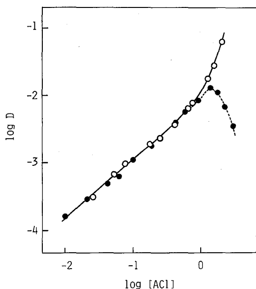
Fig. 2. The distribution ratio of manganese as a function of chloride concentration.
