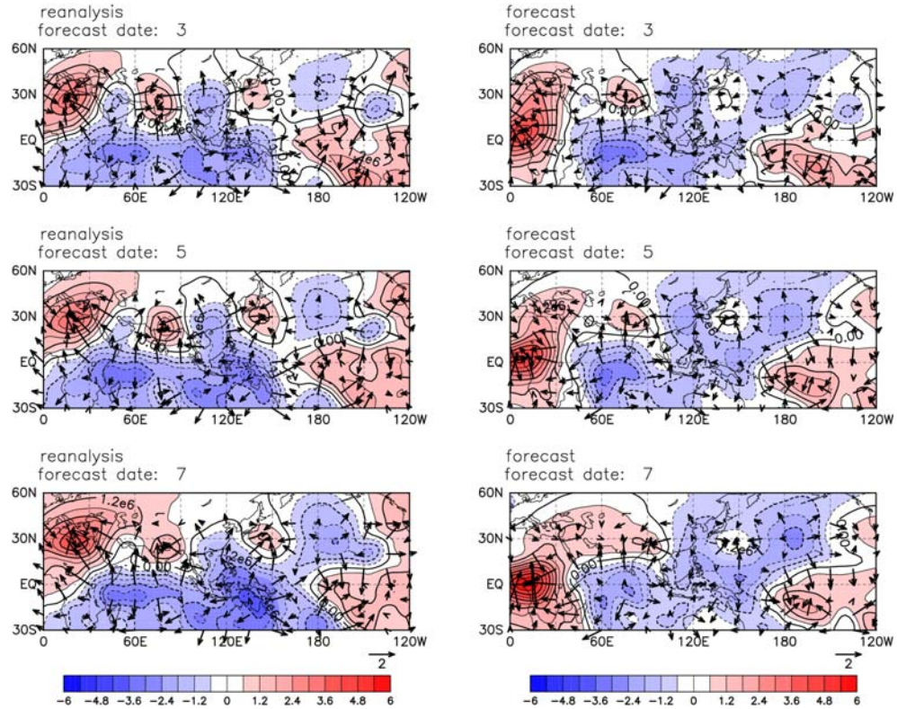
Fig. 4 As in Fig. 3, but for X200 anomalies (contour). Contour interval is 0.6 \times 10^6 \text{ m}^2/\text{s} . Negative values correspond to divergence. Arrows show corresponding divergent wind anomalies. The magnitude of the reference vector is shown in the lower right corner. Divergent winds poleward of 45N are not shown.
