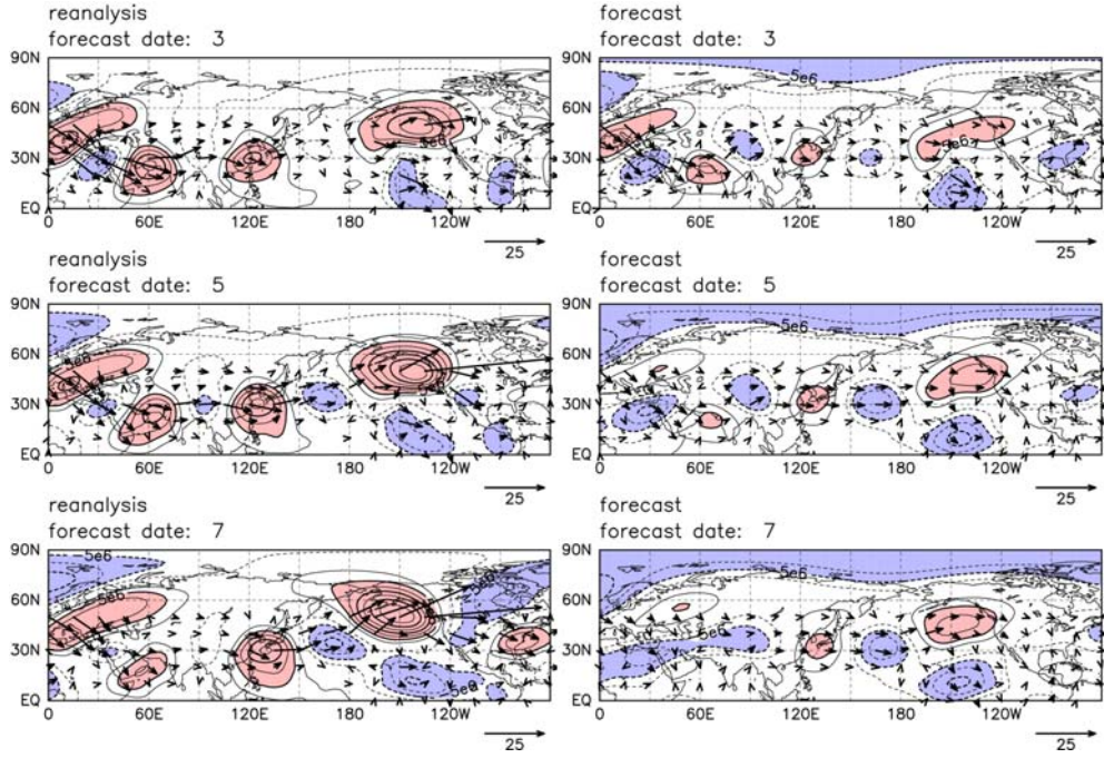
Fig. 3 Composited \phi_{200} (contour) anomalies for forecasts with large prediction error of day-7 PNA index for negative PNA events. Contour interval is 2.5 \times 10^6 \text{ m}^2/\text{s} . Regions where the magnitude of anomaly is larger than 5 \times 10^6 \text{ m}^2/\text{s} are shaded. Arrows show the corresponding wave-activity flux anomalies. The magnitude of the reference vector is shown in the lower right corner. Wave-activity fluxes poleward of 60N are not shown.
