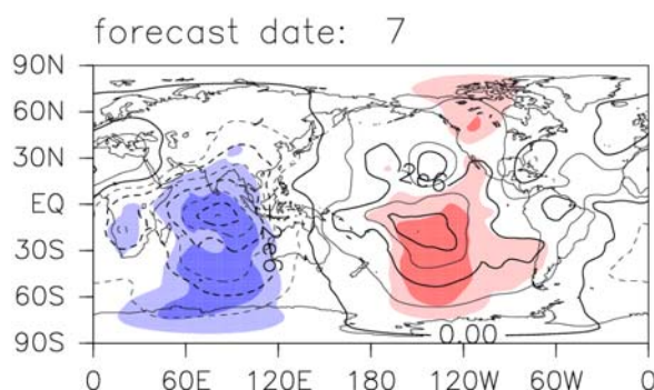
Fig. 2 Regressed 7-day averaged X200 anomaly at the initial time of forecast with respect to day-7 forecast error of PNA index for PNA events. Regions with negative anomalies correspond to divergent regions. Contour interval is 1 \times 10^6 \text{ m}^2/\text{s} . Anomalies in heavy (lightly) shaded regions are statistically significant at 99(95)% confidence level.
