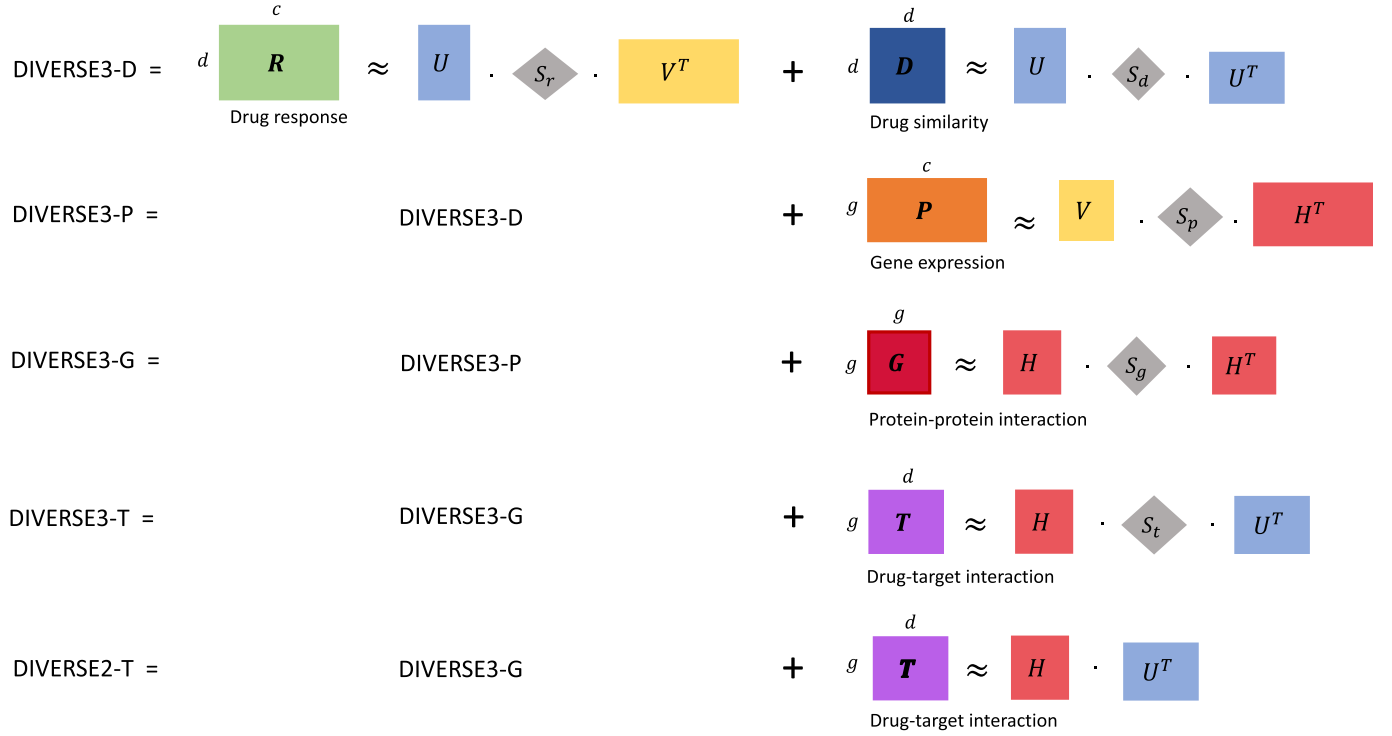
Fig. 3. Overview of our systematic framework, DIVERSE, of integrating multiple data sets: importance weight tri-(or bi-)matrix factorization. We start with adding D to R (first row: DIVERSE3-D). We then add P to DIVERSE3-D (second row: DIVERSE3-P). Similarly we add G to DIVERSE3-P (third row: DIVERSE3-G) and T to DIVERSE3-G (fourth row: DIVERSE3-T). Another option of the last addition is bi-matrix factorization, and this is the last row: DIVERSE2-T.
