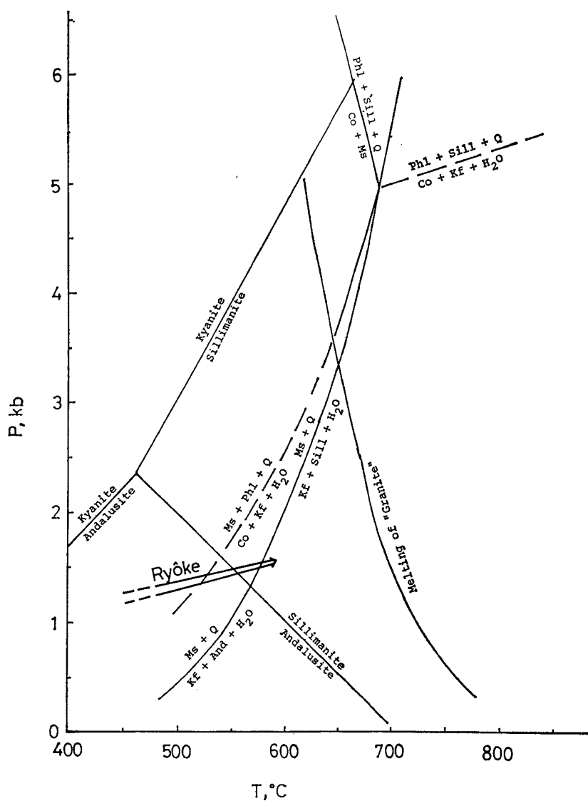
Fig. 28. Phase diagrams relevant to understanding the P-T condition of the Ryôke regional metamorphism.
