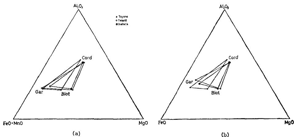
Fig. 26. Coexisting garnet, cordierite and biotite, plotted in (a) \text{Al}_2\text{O}_3 -FeO+MnO-MgO diagram, (b) \text{Al}_2\text{O}_3 -FeO-MgO diagram.
