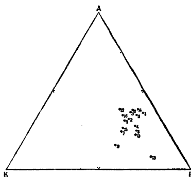
Fig. 11. AKF diagram for pelitic and psammitic metamorphic rocks in the Toyone-mura area.
