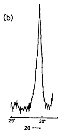
Fig. 13. 131 and \bar{1}\bar{3}1 of reflections in powder diffraction patterns of potash feldspars.
