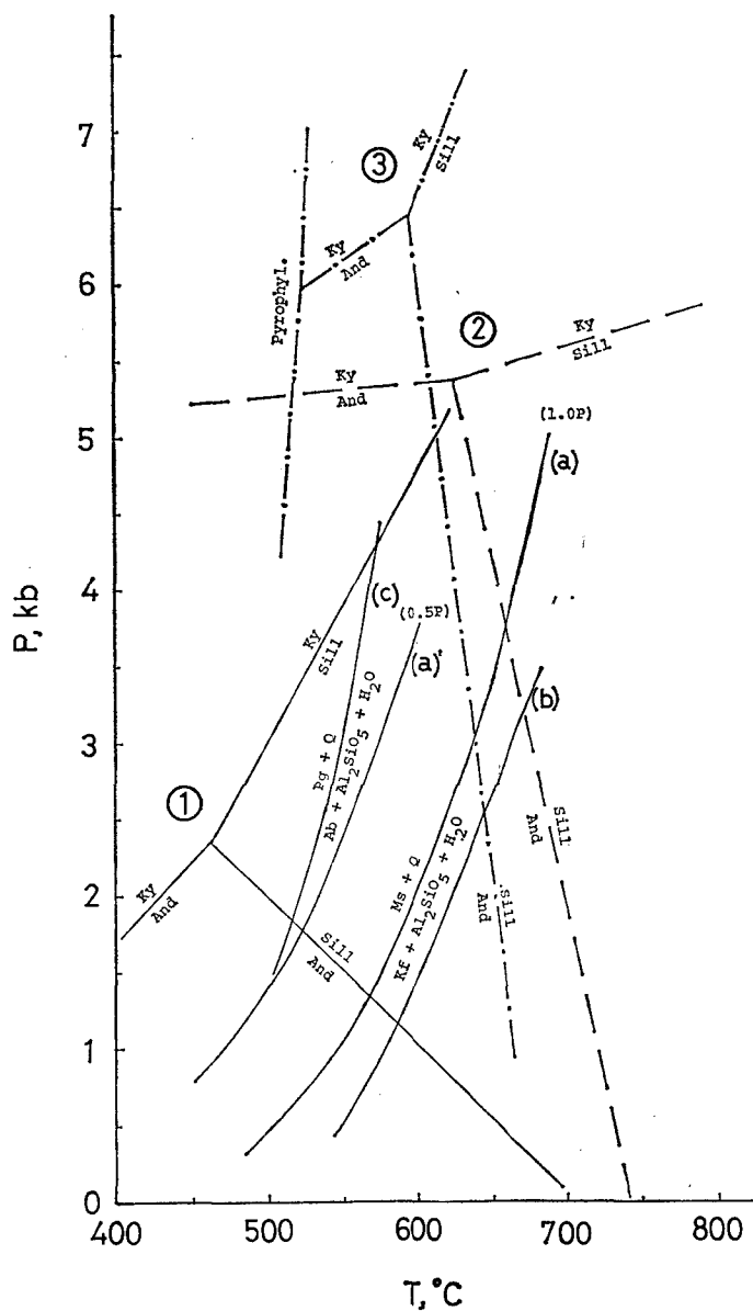
Fig. 25. Phase diagram showing stability fields of the polymorphs of \text{Al}_2\text{SiO}_5 .
