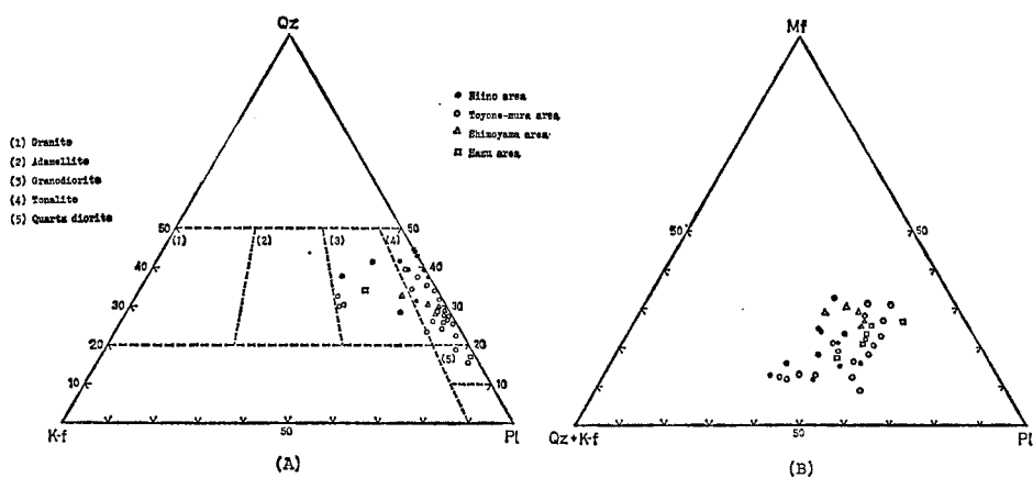
Fig. 6. (A) Modal quartz-potash feldspar-plagioclase diagram, (B) Modal total mafics-quartz plus potash feldspar-plagioclase diagram, of the Kamihara quartz diorite in the Ryôke zone of the Chûbu district.
