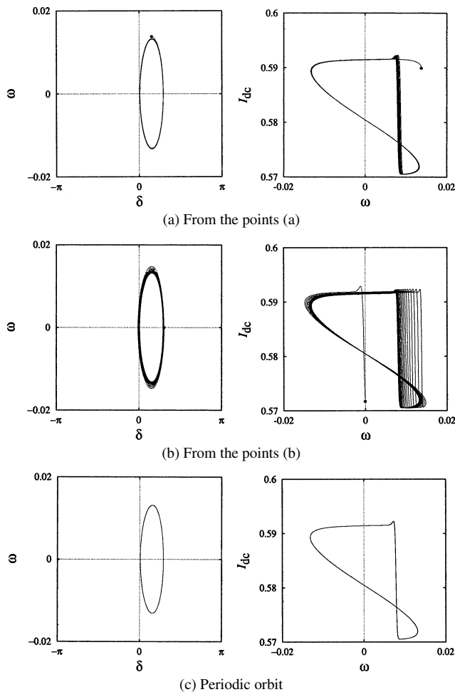
Fig. 6 Projected straddle orbits and periodic orbit in the associated SP system (16) at \varepsilon = 0.5 .
