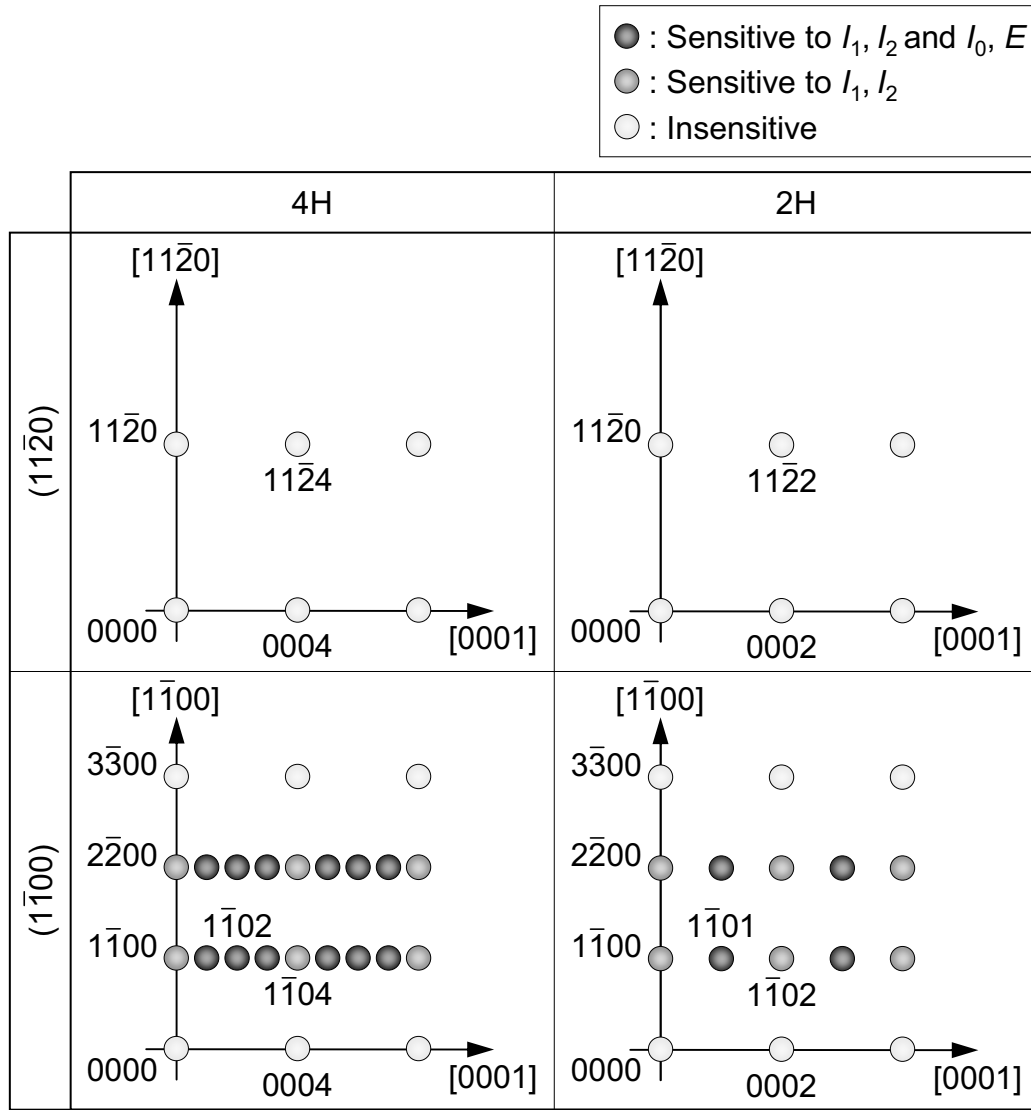
Figure 4.10: Dependence of sensitivity for XRD on the SF type and on the diffraction planes for 4H and 2H structure with [11\bar{2}0] and [1\bar{1}00] growth directions displayed in the reciprocal space.
