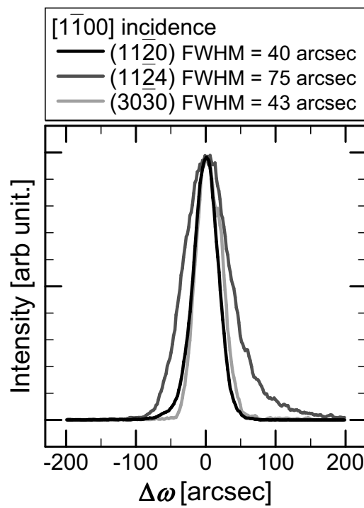
Figure 3.10: XRD \omega -scan spectra for the optimized 4H-AlN layer grown on 4H-SiC (11̄20). Symmetrical (11̄20) and asymmetrical (11̄24) and (3030) reflections are shown. The x-ray incident geometry parallel to [11̄00] was used.
