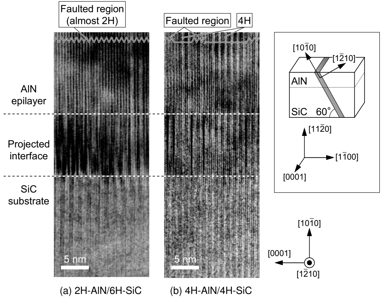
Figure 1.7: Cross-sectional high-resolution TEM images of (a) 2H-AlN/6H-SiC ( 11\bar{2}0 ) and (b) 4H-AlN/4H-SiC ( 11\bar{2}0 ) interfaces [74]. The inset shows the geometry of TEM specimens. In the upper of the TEM images, the regions of 4H structures and faulted region are shown by straight and notched lines, respectively.
