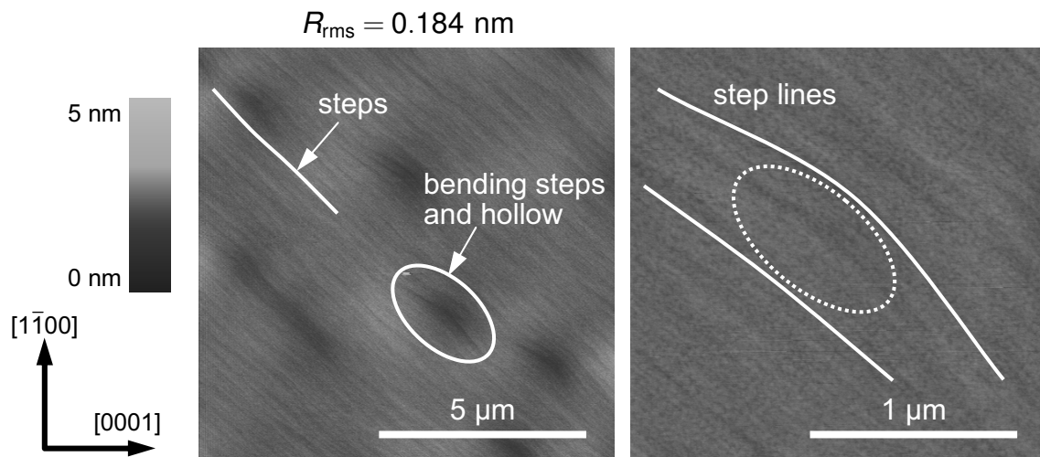
Figure 6.5: Surface morphologies of 4H-SiC ( 11\bar{2}0 ) after the annealing at a high temperature of 1600°C for 15 min. The solid lines show the guide of the step edge to the eye and the ellipses indicate a hollow. A hollow observed in left image is magnified to the right one.
