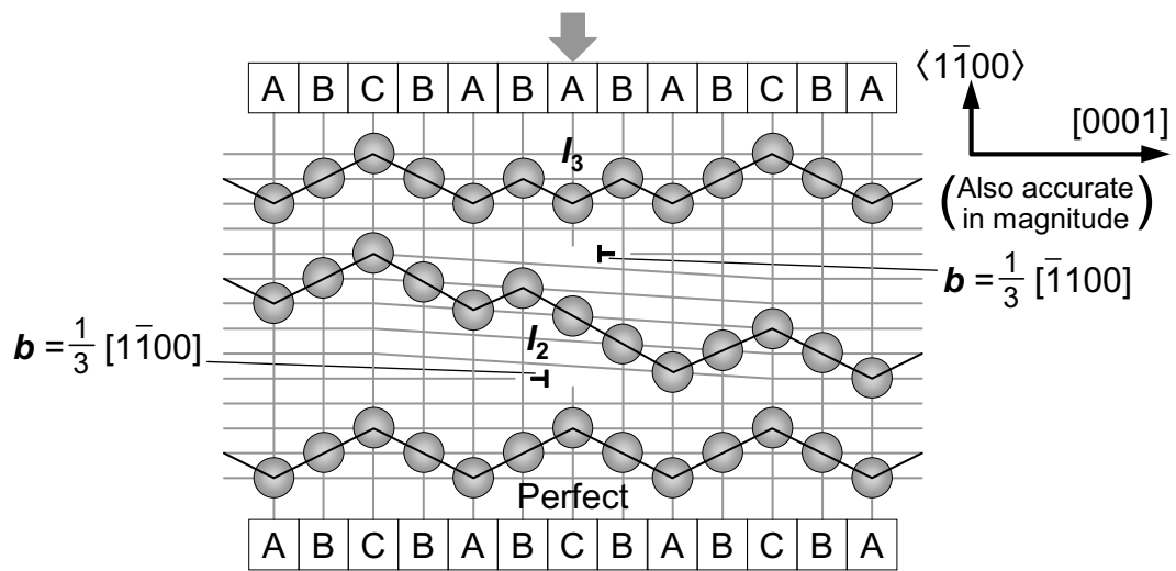
Figure 4.7: Structure schematics that two partial dislocations of the I_2 type form the same SF as the I_3 type in 4H-polytype structure. The dislocations travel from the front side to the back side of the page.
