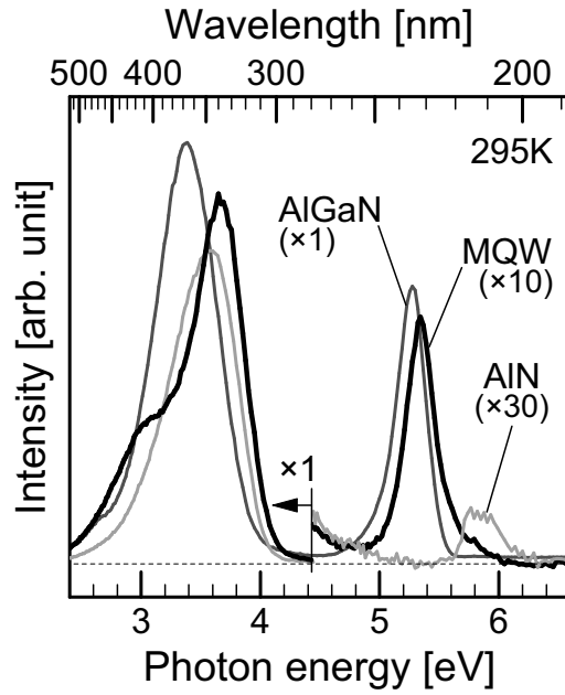
(a) CL spectra from MQW, AlGa 0.10 N and AlN layers (RT)
