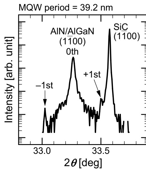
Figure 5.11: An XRD 2\theta/\omega -scan spectrum of (1\bar{1}00) reflections obtained from 23-nm-thick AlN/16-nm-thick AlGaN MQW structure grown on 4H-SiC (1\bar{1}00) . The period of MQW structure is estimated from the interval of the satellite peaks.
