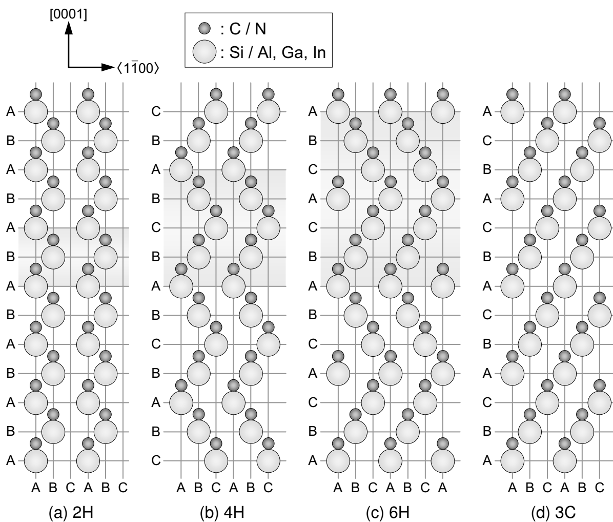
Figure 1.3: Stacking orders along [0001] ( c -axis) for (a) 2H-, (b) 4H-, (c) 6H- and (d) 3C-structures of SiC or III-Ns.
