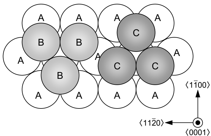
Figure 1.2: Hexagonal closed packing of Si-C or III-N pairs.
