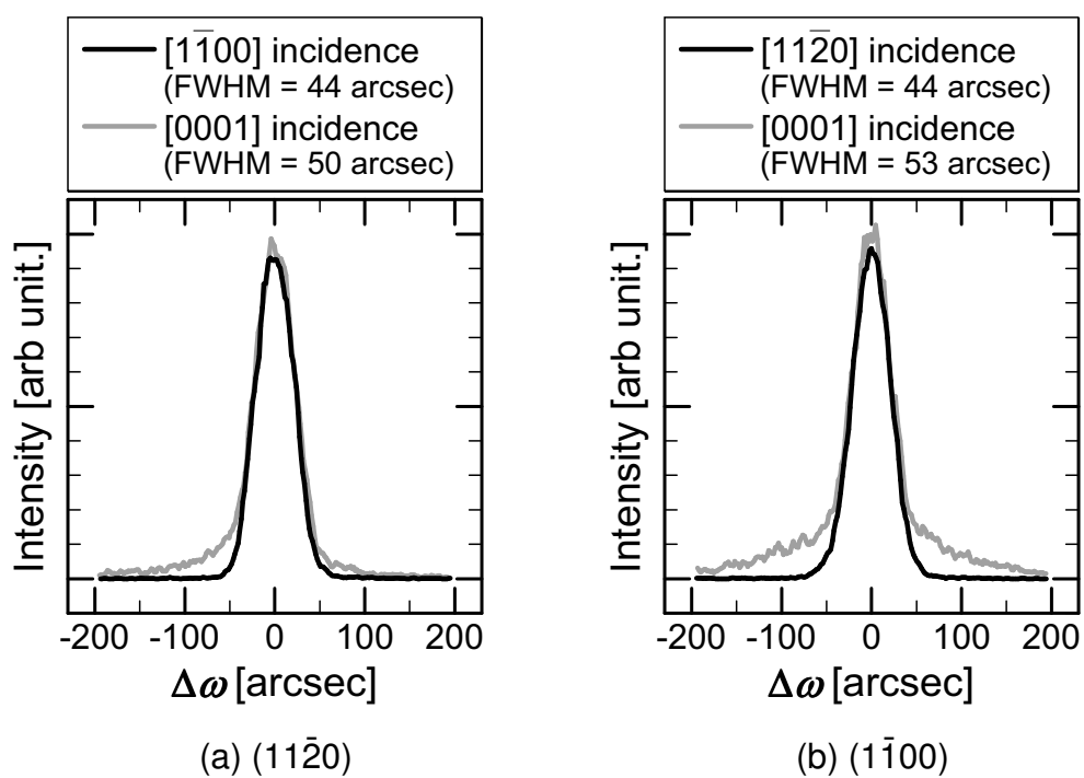
Figure 4.8: XRD \omega -scan spectra of 4H-AlN (a) (11\bar{2}0) and (b) (11\bar{0}0) measured with the different x-ray incidence.
