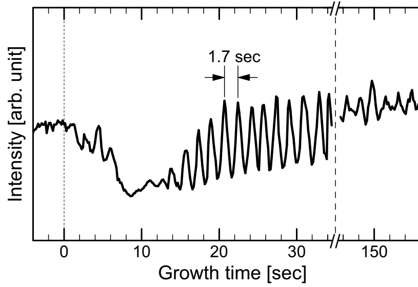
Figure 3.17: A RHEED intensity profile of a 1\bar{1}00 streak observed during initial growth of 4H-AlN on 4H-SiC ( 1\bar{1}00 ) at the growth temperature of 750°C. The profile is also shown in the growth time around 150 sec ( \sim 90 th cycle).
