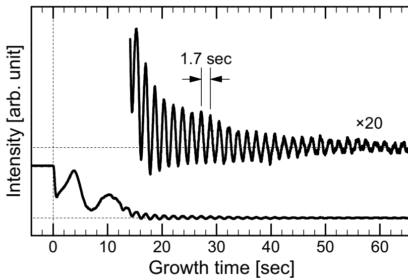
Figure 5.5: RHEED intensity profiles during the initial stage of AlGaIn growth. The profiles are shown in the whole amplitude and the magnified amplitude.
