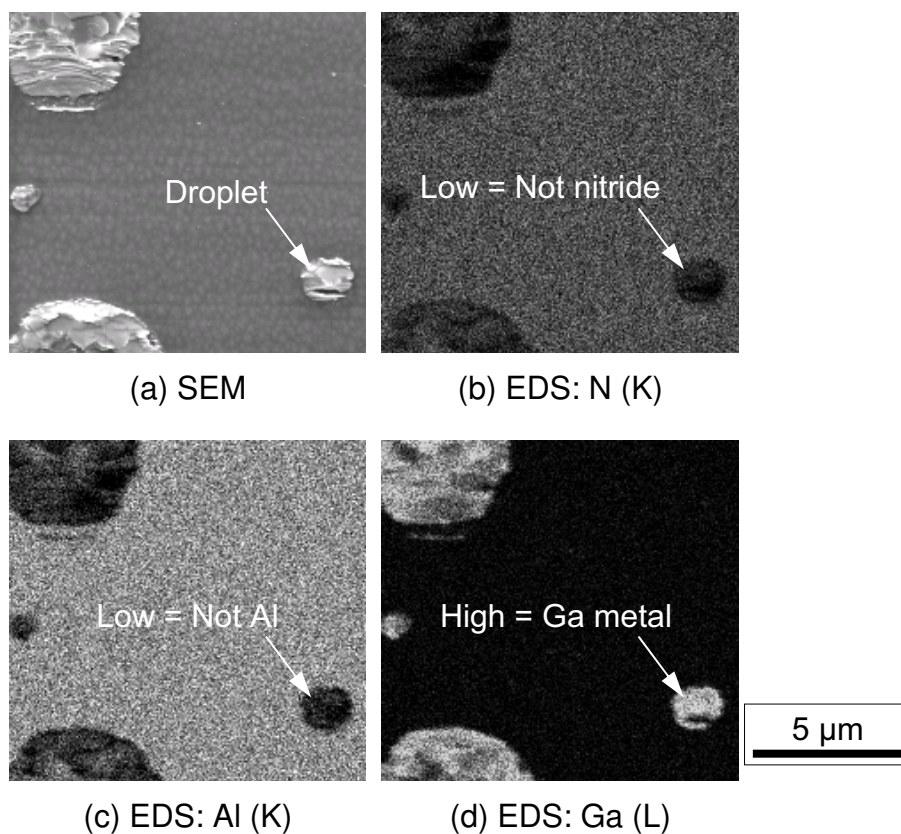
Figure 5.1: (a) an SEM image and EDS mapping images of (b) N (K-line), (c) Al (K-line) and (d) Ga (L-line) taken from Al(Ga)N ( 11\bar{2}0 ) layers grown at 750°C under the Ga BEP ratio of 0.66. In the EDS mapping images, the brightness displays the weight ratio.
