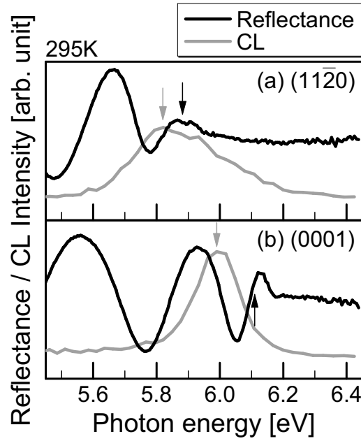
Figure 4.14: Spectra of optical reflectance (black) and cathodoluminescence (CL) (gray) from (a) 4H-AlN ( 11\bar{2}0 ) and (b) 2H-AlN (0001). The black arrows show the absorption edges of E_A and the gray arrows show the CL peaks from bound excitons.
