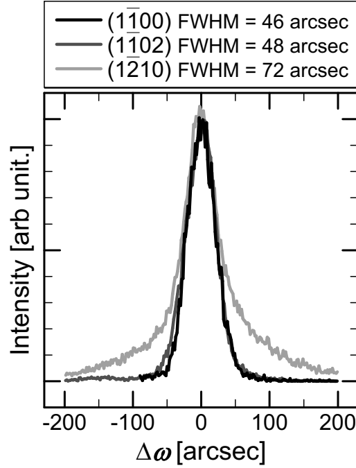
Figure 5.6: XRD \omega -scan spectra of 4H-Al 0.9 Ga 0.1 N ( 1\bar{1}00 ) grown on 4H-SiC ( 1\bar{1}00 ). Symmetrical ( 1\bar{1}00 ) and asymmetrical ( 10\bar{1}2 ) and ( 1\bar{2}10 ) reflections are shown. ( 1\bar{1}00 ) and ( 10\bar{1}2 ) reflections are obtained in x-ray incident geometry parallel to the [11\bar{2}0] direction, and a ( 1\bar{2}10 ) reflection parallel to the [0001] direction.
