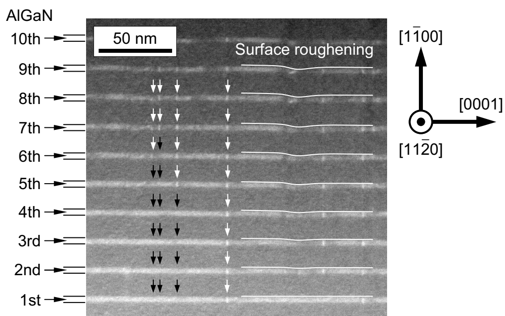
Figure 5.14: A Z (atomic weight) contrast image observed in HAADF STEM of 15-nm-thick AlN/4-nm-thick AlGa N MQW structures. The white arrows show the bright stripes observed and the black arrows show no observation of stripes in each AlGa N layer. The shapes of AlN/AlGa N interfaces are shown by the solid lines.
