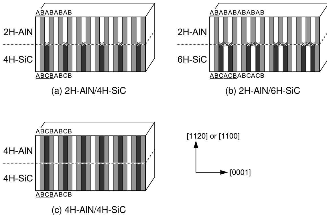
Figure 1.6: Schematic illustration of polytype mismatch between nonpolar (a) 2H-AlN/4H-SiC, (b) 2H-AlN/6H-SiC and (c) 4H-AlN/4H-SiC. The cross indices indicate partial dislocations extended perpendicularly to the page.
