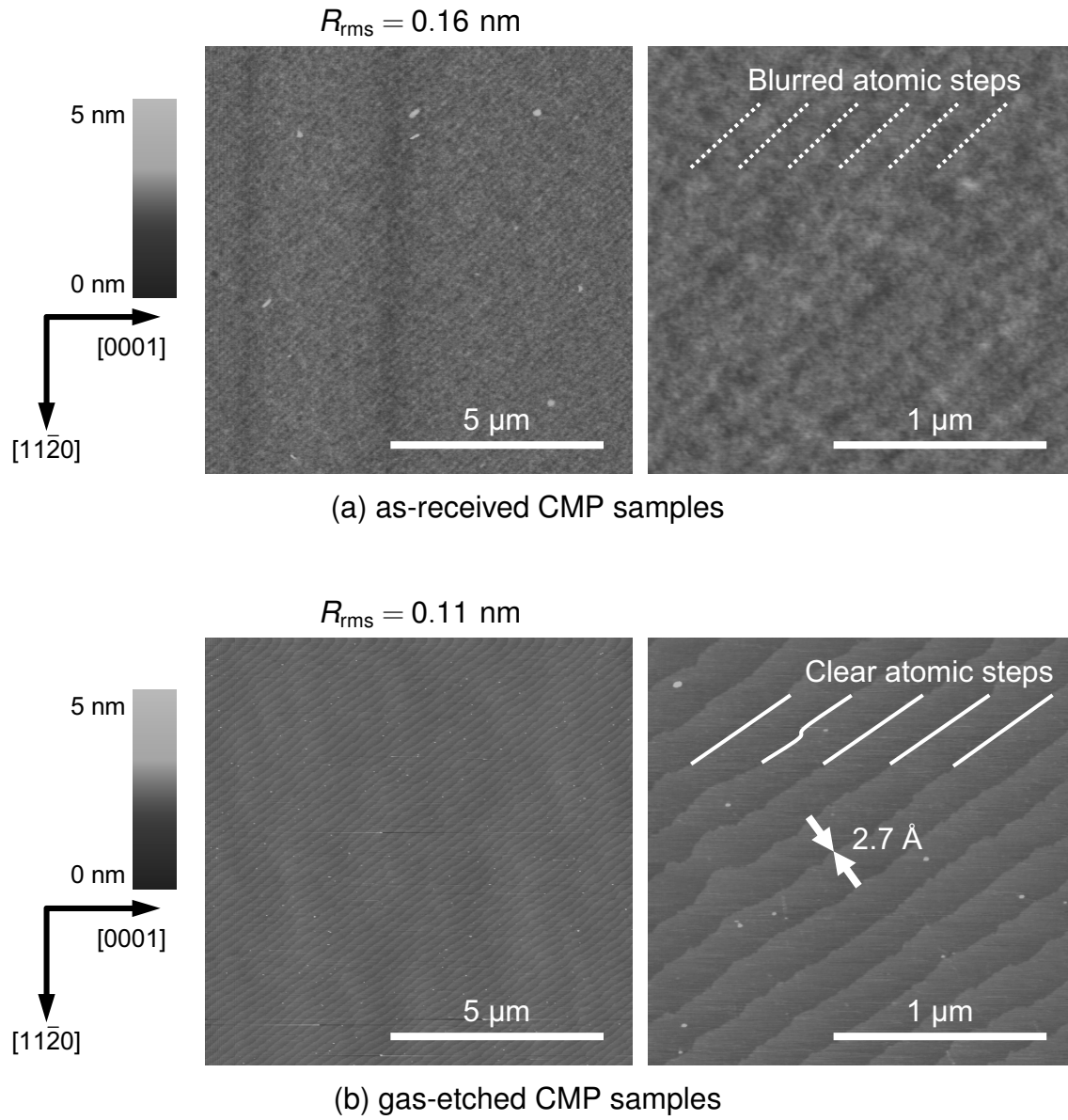
Figure 2.9: Surface morphologies of 4H-SiC (1100): (a) as-received CMP samples and (b) gas-etched CMP samples. Each of right figures shows a magnified image of the left one.
