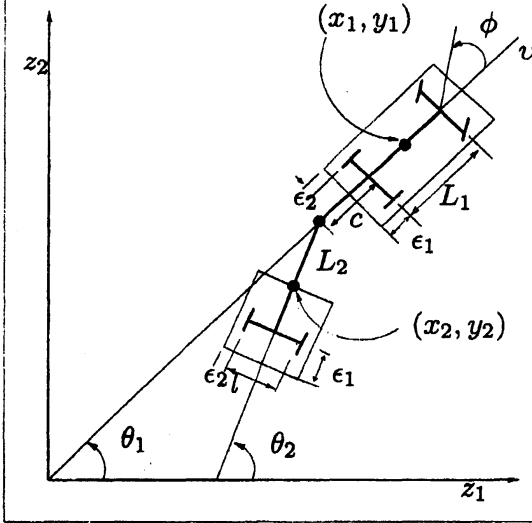
Figure 1: Kinematic model of a general 1-trailer robot
