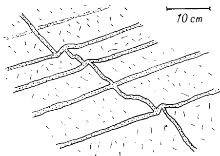
Fig. 2. Deformation of sandstone beds at the points of connection with a dike. Boundary between the dike and the sandstone beds is invisible. Loc. 2.
