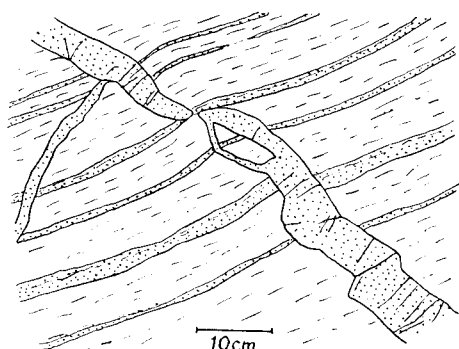
Fig. 3. Dike having a branch and a captured country rock. Loc. 4.
