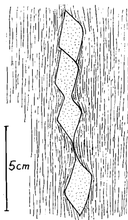
Fig. 6. Thin dike deformed into lozenge-shaped segments. The figure represents the cross-joint surface perpendicular to the axis of main fold. Loc. 8.
