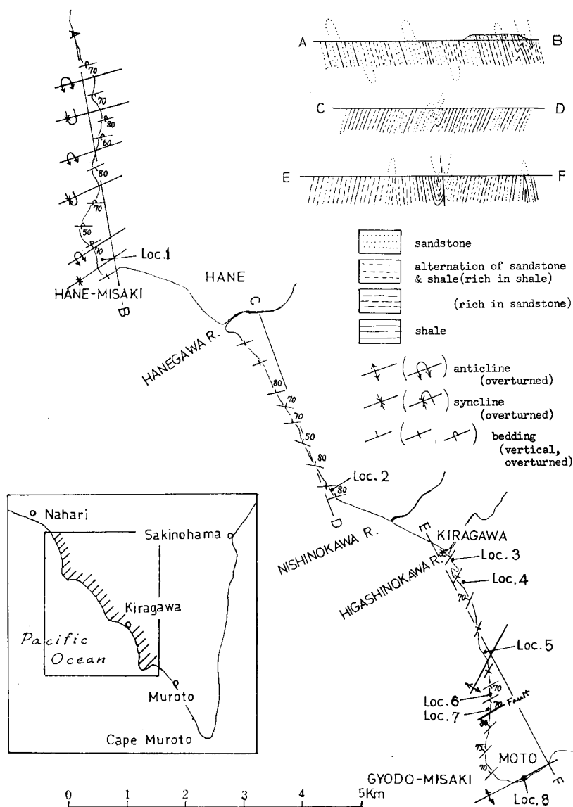
Fig. 1. Geologic profiles and distribution of the dikes along part of the western coast of the Muroto district.
