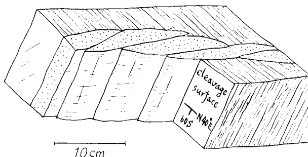
Fig. 7. Diagrammatic figure showing a dike cut into lenses of which edges are nearly parallel to the dip direction of the cleavage surface.
