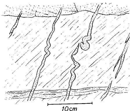
Fig. 4. Parallel-running dikes which make a definite angle with bedding plane. Loc. 7.
