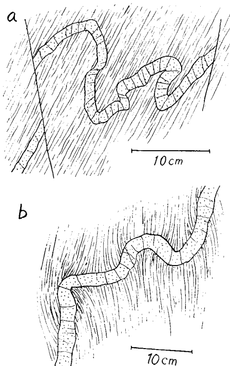
Fig. 5. a. Folded dike not related to cleavage development in shale. b. Dike showing an influence of its folding on the development of cleavage. Loc. 8.
