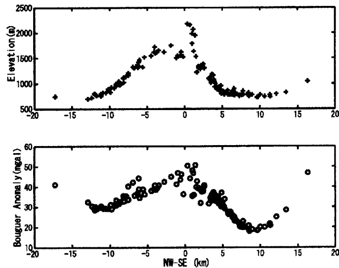
Fig.6-2 Profile of Bouguere anomaly in NW-SE direction (lower figure) and elevation of gravity station (upper figure). Area of data is shown in Fig.6-1.
