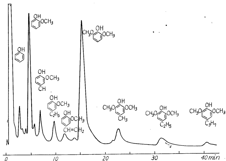
Fig. 4. Pyrolytic Gaschromatogram of SAKURA Wood Thiolignin.
