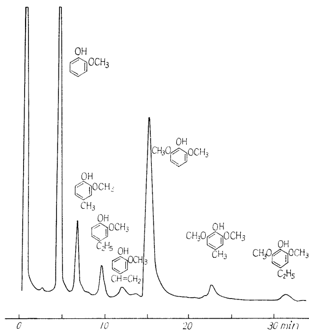
Fig. 2. Pyrolytic Gaschromatogram of BUNA Wood Thiolignin.
