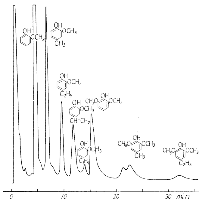
Fig. 3. Pyrolytic Gaschromatogram of MOKKOKU Wood Thiolignin.
