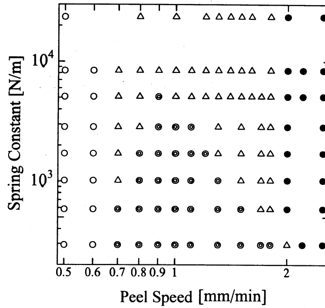
Figure 7: Dynamical-morphological phase diagram in V-k space.
