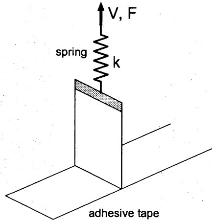
Figure 1: Schematic representation of the experimental setup.
