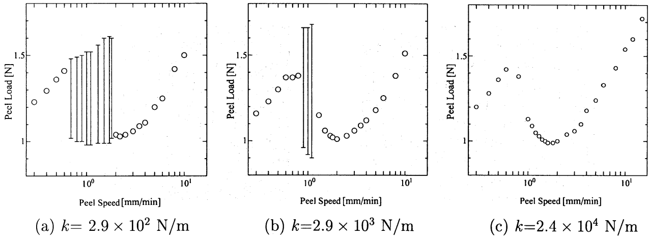
Figure 2: Peel load as a function of peel speed V in three cases with a different spring constant. (a) k = 2.9 \times 10^2 \text{ N/m} , (b) k = 2.9 \times 10^3 \text{ N/m} , (c) k = 2.4 \times 10^4 \text{ N/m} . The bar represents the amplitude of the oscillatory motion in peel load at each fixed peel speed.
