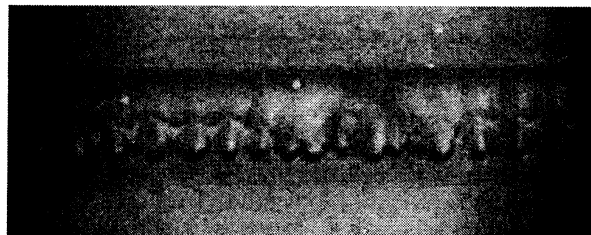
Figure 8: A failure front in the case of a spatio-temporal intermittent pattern. Two kinds of failure morphologies, namely, morphologies in low-speed pattern and high-speed pattern coexist. The actual size of this figure is 1.9 \text{ mm} \times 0.75 \text{ mm} .
