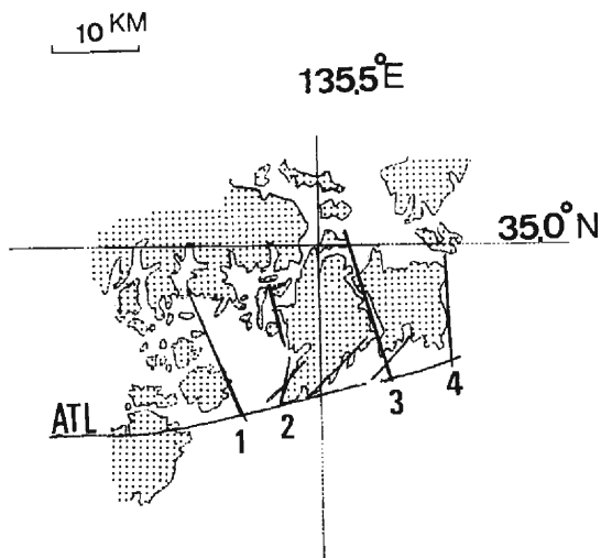
Fig. 24 Topography around the ATL. Contours indicate 300 m height and hatched area is higher than 300 m. The lines attached by numerals represent boundaries of blocks. These lines coincide with the rivers shown in Fig 23.
