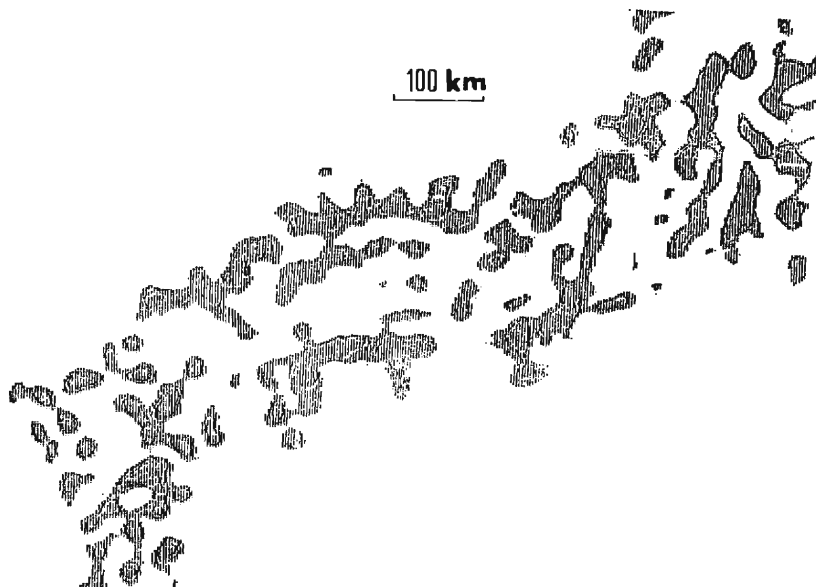
Fig. 8-a Pattern of topography extracted by a band-pass filter with a central wavelength of 40 km. Band width is between 20–90 km. Shadow part indicates positive area corresponding to upheaval region. White area indicates negative area.
