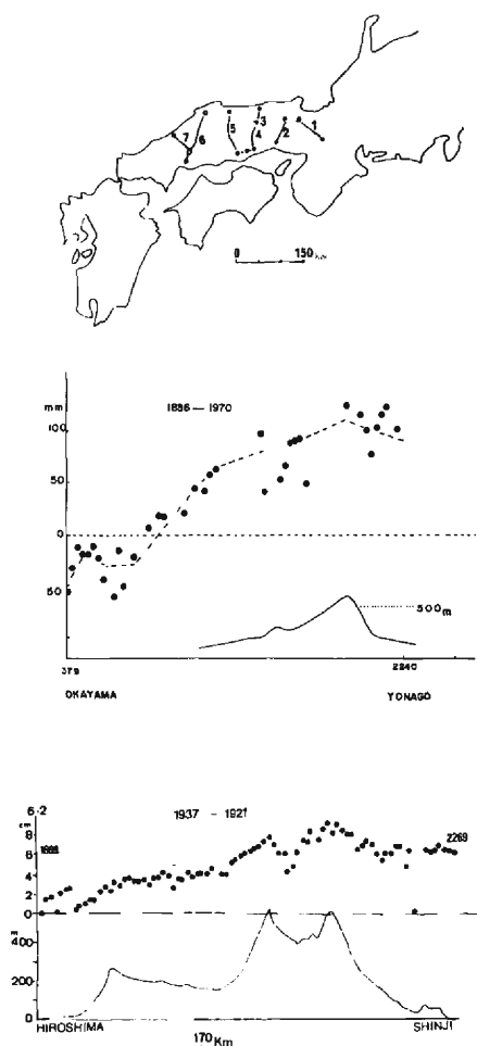
Fig. 9. Routes and results of leveling surveys across the Chugoku mountains Upperr: the routes of leveling surveys Middle: result of leveling survey and topography along route No. 5 Lower: result of leveling survey and topography along route No. 6
