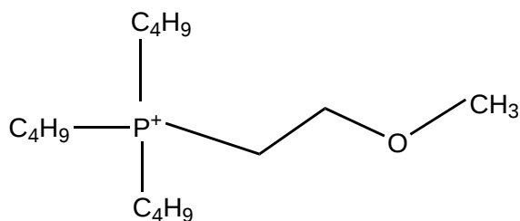
Tributyl(2-methoxyethyl)phosphonium (TBMOP + )
