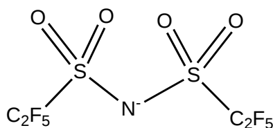
Bis(pentafluoroethanesulfonyl)amide (C 2 F 5 SO 2 ) 2 N - )
