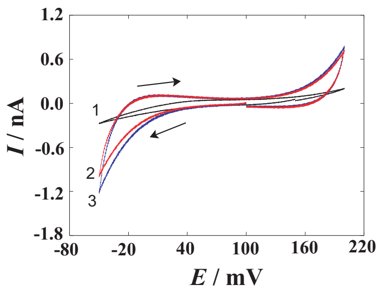
Figure 6.17: Cyclic voltammograms for the 0.12 \text{ mol kg}^{-1} NaCl (Curve 1), 1:2 HEPES (Curve 2), 1:2 TES (Curve 3) in W1 in cell (B). The scan rate: 50 \text{ mV s}^{-1} . Arrows by the line indicate the direction of the scanning.
