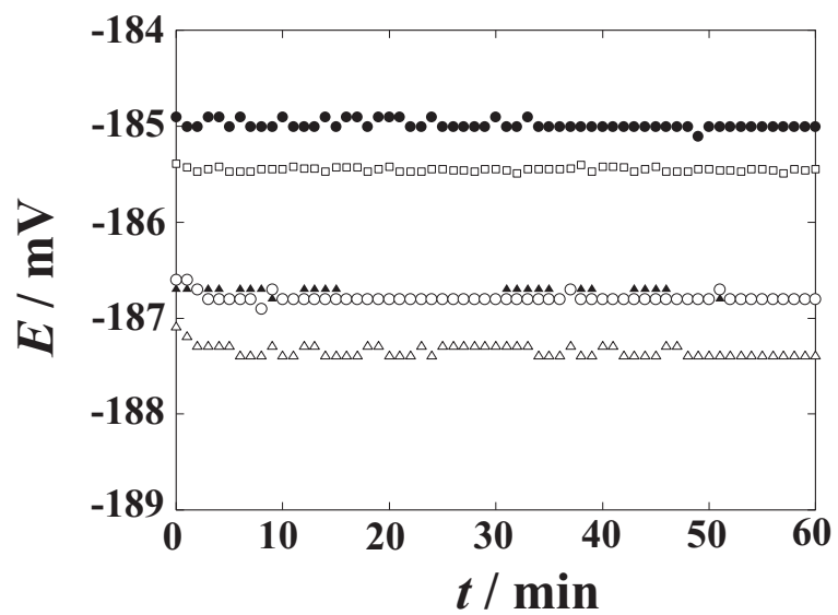
Figure 4.5: Time dependence of E for 1 h at 0.025 \text{ mol kg}^{-1} equimolal phosphate buffer solutions in cell (A) at 60^\circ\text{C} . \circ : 1st measurement, \triangle : 2nd measurement, \square : 3rd measurement, \bullet : 4th measurement, \blacktriangle : 5th measurement.
