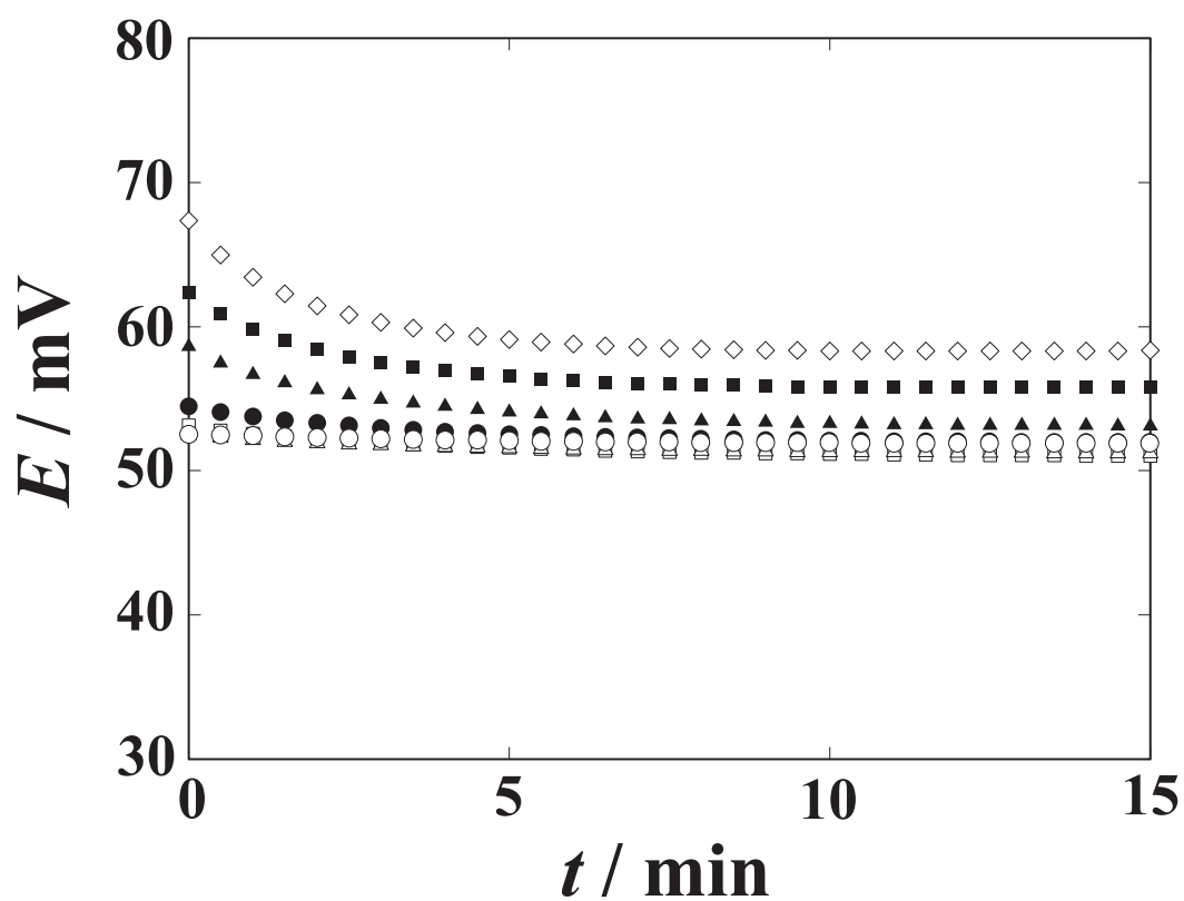
Figure 5.6: Time dependence of E for 15 min at 0 ~ 0.2 mol dm -3 KHPH in IV and C 6 mimCl in II and C 6 mimC 2 C 2 N in III in cell (C). ○ : 0 mol dm -3 , △ : 0.001 mol dm -3 , □ : 0.005 mol dm -3 , ● : 0.01 mol dm -3 , ▲ : 0.05 mol dm -3 , ■ : 0.1 mol dm -3 , ◇ : 0.2 mol dm -3 .
