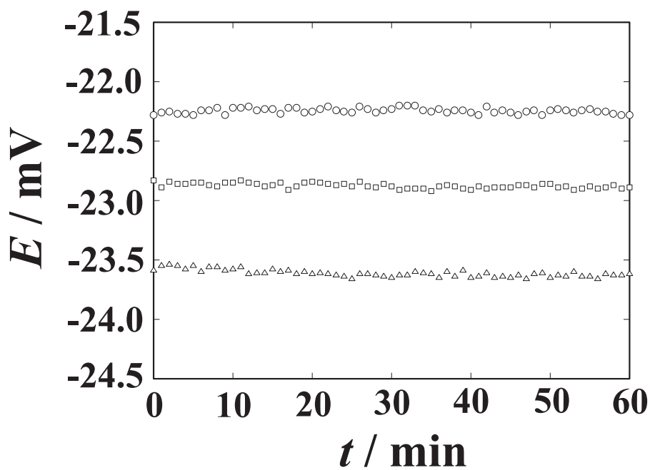
Figure 1.6: Time dependence of E for 1 h at 200 \mu\text{mol dm}^{-3} \text{H}_2\text{SO}_4 solution in cell (A). Open circle : first measurement, open triangle : second measurement, open square: third measurement.
