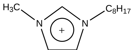
1-Methyl-3-octylimidazolium ( \text{C}_8\text{mim}^+ )
