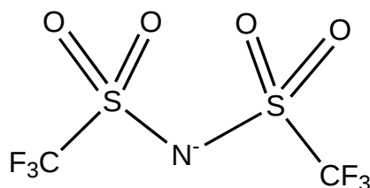
Bis(trifluoromethanesulfonyl)amide ( \text{C}_1\text{C}_1\text{N}^- )
