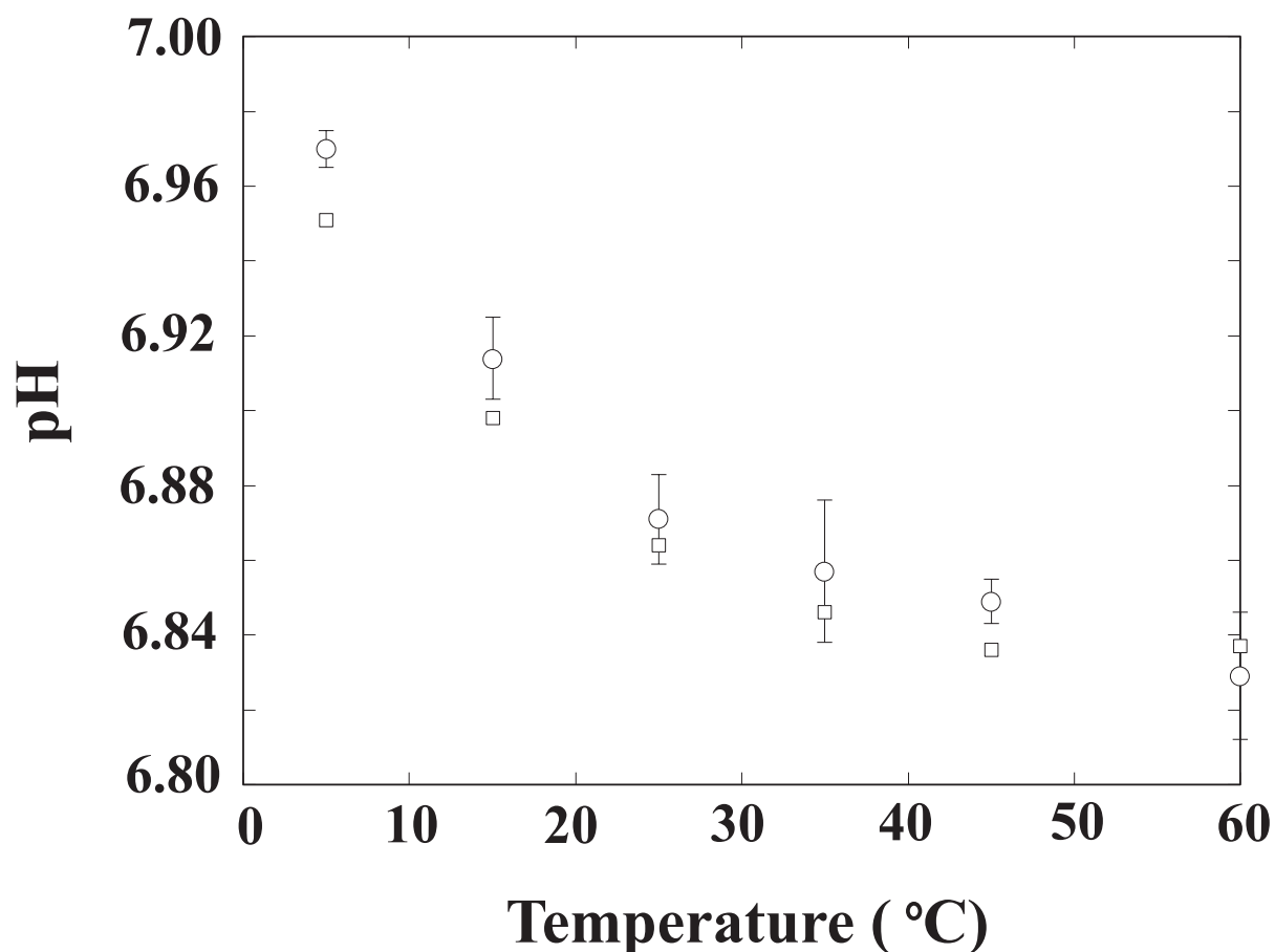
Figure 4.6: Experimental pH values (○) obtained by use of the ILSB and pH values obtained by a Harned cell (□) at 0.025 mol kg -1 equimolal phosphate buffer solutions at 5 - 60 °C.
