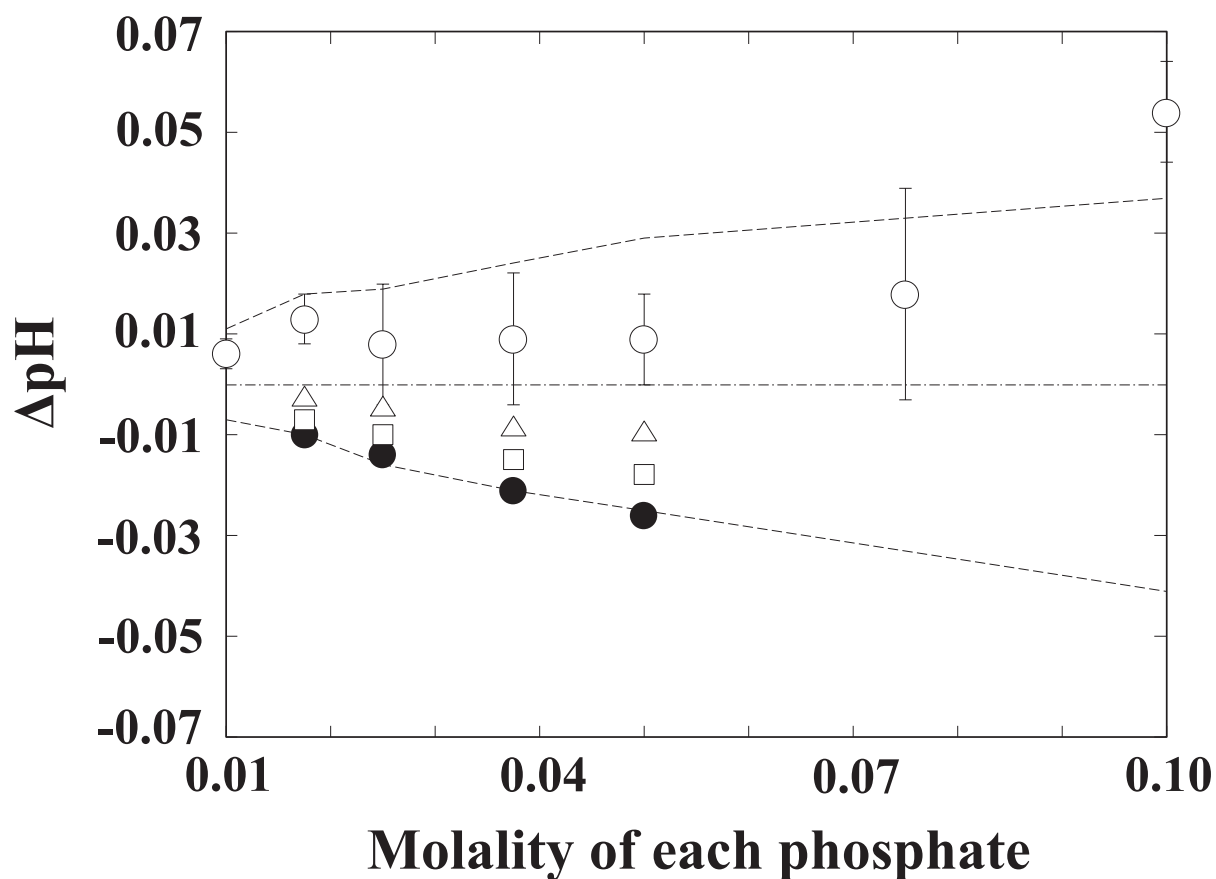
Figure 3.9: Difference between experimental pH values (○) obtained by use of the ILSB and the calculated pH values with the Pitzer equation at 0.01 ~ 0.1 mol kg -1 equimolal phosphate buffer solutions. Difference between pH values obtained by Harned cells with silver chloride (Δ), silver bromide (□), or silver iodide (●) electrodes and the calculated pH values with the Pitzer equation. The dashed lines indicate the curve of the difference between pH values for \gamma values of 8 (upper line) or 3 (lower line) and the calculated pH values with the Pitzer equation.
