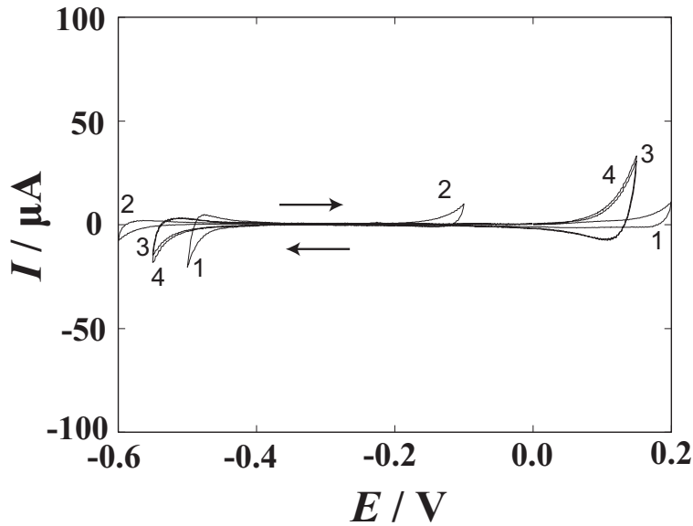
Figure 6.12: Cyclic voltammograms for the 10 mM \text{Li}_2\text{SO}_4 (Curve 1), 10 mM \text{Li}_2\text{SO}_4 + 50 mM Tris-HCl (Curve 2), 10 mM \text{Li}_2\text{SO}_4 + 60 mM HEPES + 60 mM LiOH (Curve 3), and 10 mM \text{Li}_2\text{SO}_4 + 60 mM TES + 60 mM LiOH (Curve 4) in W1 in cell (B). The scan rate: 10 \text{mV s}^{-1} . Arrows by the line indicate the direction of the scanning.
