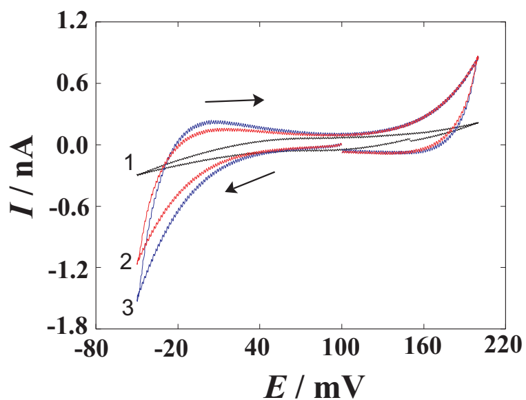
Figure 6.18: Cyclic voltammograms for the 0.12 \text{ mol kg}^{-1} NaCl (Curve 1), 1:2 HEPES (Curve 2), 1:2 TES (Curve 3) in W1 in cell (B). The scan rate: 100 \text{ mV s}^{-1} . Arrows by the line indicate the direction of the scanning.
