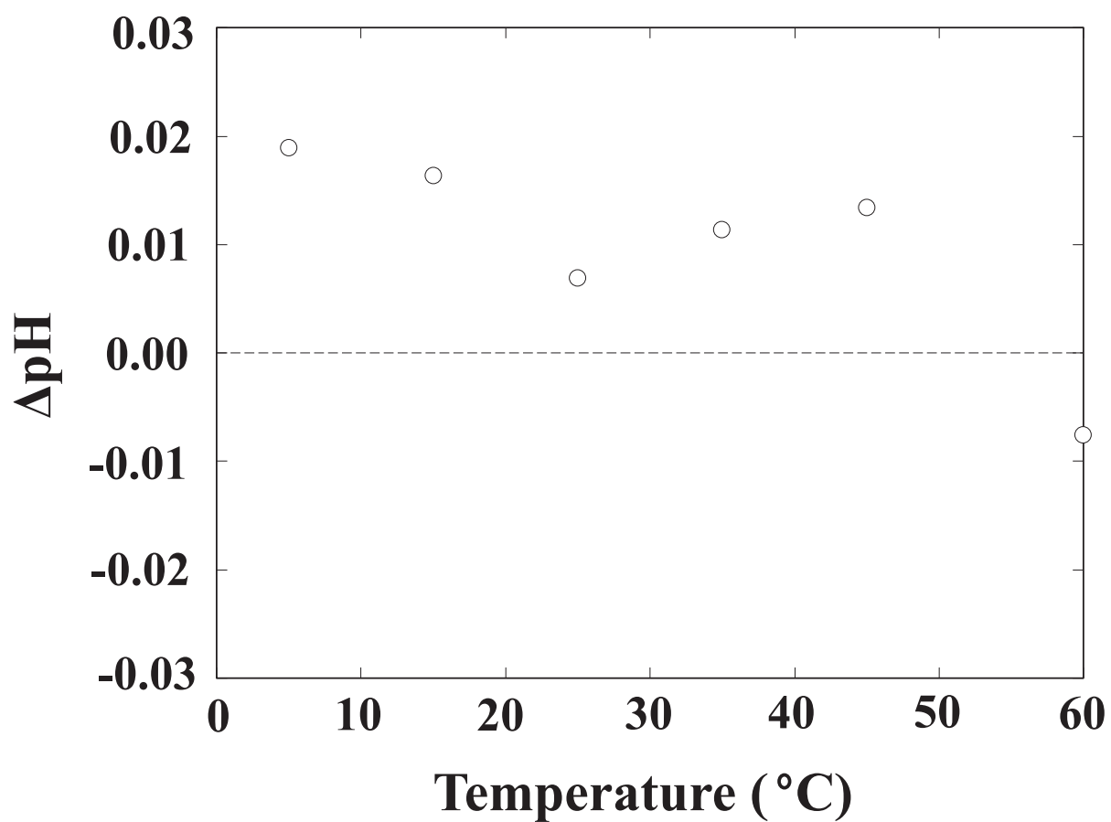
Figure 4.7: Difference between experimental pH values obtained by use of the ILSB and pH values obtained by a Harned cell at 0.025 mol kg -1 equimolal phosphate buffer solutions at 5 - 60 °C. \Delta\text{pH} = \text{pH}_{\text{ex}} - \text{pH}_{\text{Harned}} .
