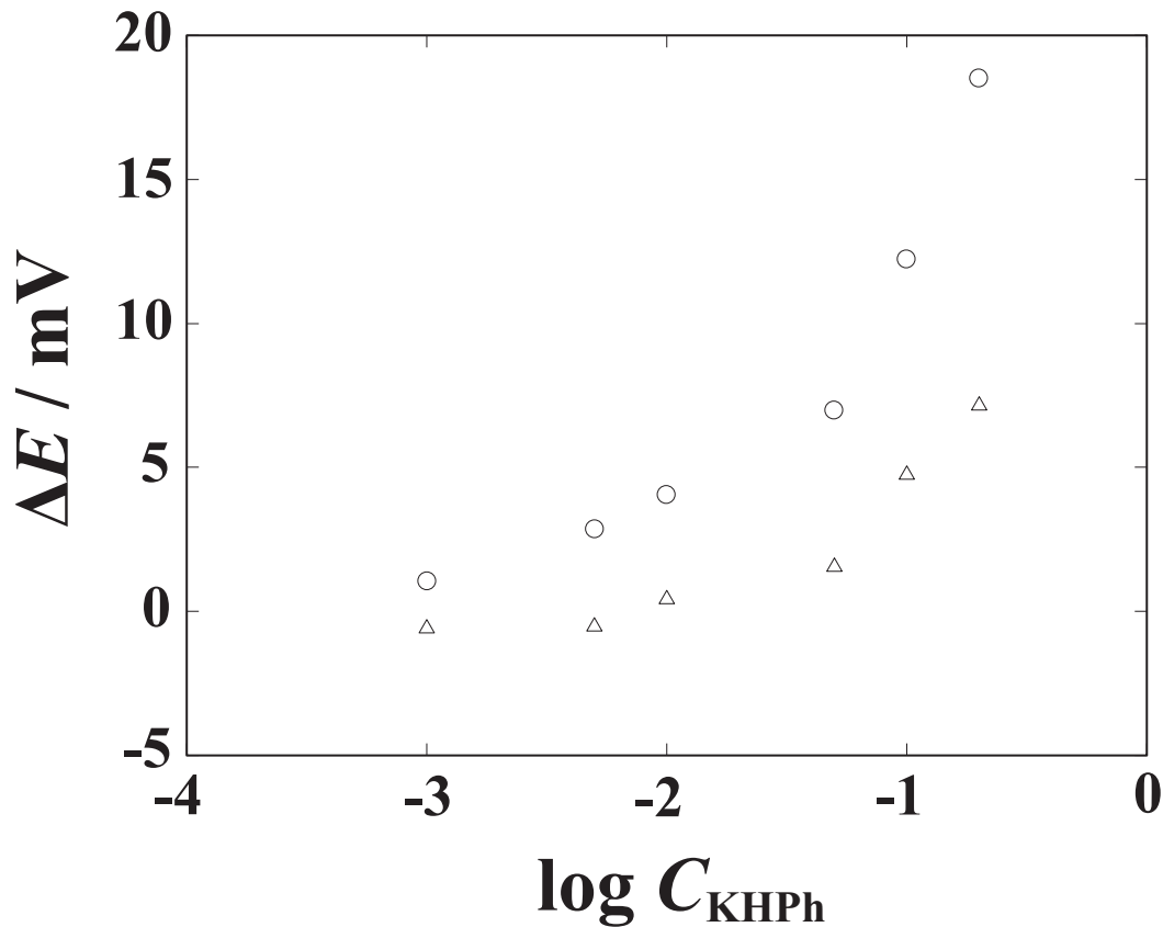
Figure 5.7: Difference between the values of E at each concentration of KHPH and the value of E at zero concentration of KHPH in IV in cell (C) for 0.001 \sim 0.2 \text{ mol dm}^{-3} KHPH.
