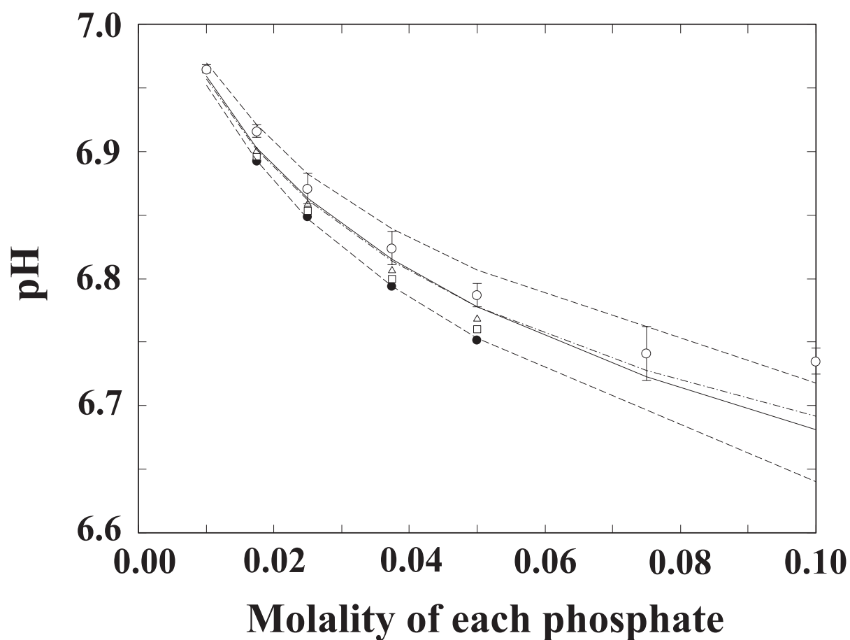
Figure 3.8: Experimental pH values (○) obtained by use of the ILSB, pH values obtained by Harned cells with silver chloride (Δ), silver bromide (□), and silver iodide (●) electrodes, and calculated pH values obtained from the Hückel equation (dashed-dotted line) and Pitzer equation (solid line) at 0.01 ~ 0.1 mol kg -1 equimolal phosphate buffer solutions. The dashed lines indicate the course of the curve of pH values for activity coefficients of 8 (upper line) and 3 (lower line).
