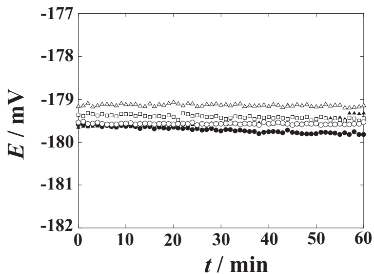
Figure 4.4: Time dependence of E for 1 h at 0.025 \text{ mol kg}^{-1} equimolal phosphate buffer solutions in cell (A) at 45^\circ\text{C} . \circ : 1st measurement, \triangle : 2nd measurement, \square : 3rd measurement, \bullet : 4th measurement, \blacktriangle : 5th measurement.
