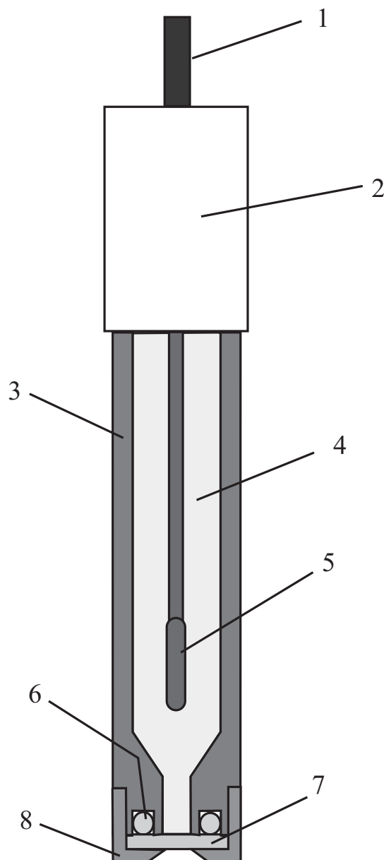
Figure 5.1: Schematic view of the ionic liquid-type reference electrode. 1, lead wire; 2, cap; 3, plastic tube; 4, 3.3 \text{ mol dm}^{-3} \text{ KCl} aqueous solution; 5, Ag/AgCl electrode; 6, O-ring; 7, gelled ionic liquid; 8, cylindrical cap
