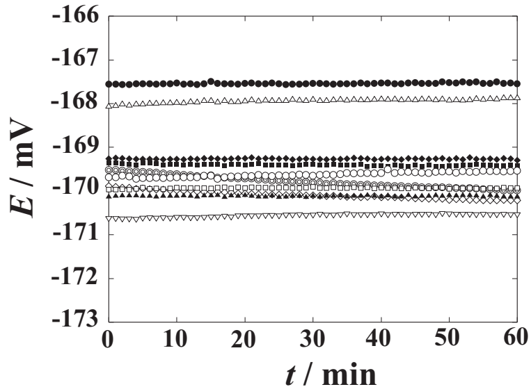
Figure 3.3: Time dependence of E for 1 h at 0.025 \text{ mol kg}^{-1} equimolal phosphate buffer solutions in cell (A). \circ : 1st measurement, \triangle : 2nd measurement, \square : 3rd measurement, \bullet : 4th measurement, \blacktriangle : 5th measurement, \blacksquare : 6th measurement, \diamond : 7th measurement, \blacklozenge : 8th measurement, \odot : 9th measurement, \nabla : 10th measurement.
