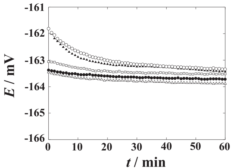
Figure 4.1: Time dependence of E for 1 h at 0.025 \text{ mol kg}^{-1} equimolal phosphate buffer solutions in cell (A) at 5 °C. ○ : 1st measurement, △ : 2nd measurement, □ : 3rd measurement, ● : 4th measurement, ▲ : 5th measurement.
