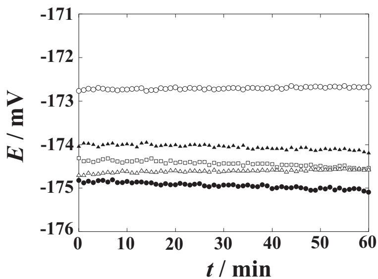
Figure 4.3: Time dependence of E for 1 h at 0.025 \text{ mol kg}^{-1} equimolal phosphate buffer solutions in cell (A) at 35^\circ\text{C} . \circ : 1st measurement, \triangle : 2nd measurement, \square : 3rd measurement, \bullet : 4th measurement, \blacktriangle : 5th measurement.
