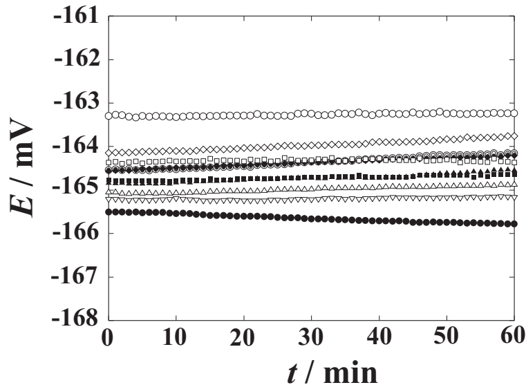
Figure 3.5: Time dependence of E for 1 h at 0.05 \text{ mol kg}^{-1} equimolal phosphate buffer solutions in cell (A). \circ : 1st measurement, \triangle : 2nd measurement, \square : 3rd measurement, \bullet : 4th measurement, \blacktriangle : 5th measurement, \blacksquare : 6th measurement, \diamond : 7th measurement, \blacklozenge : 8th measurement, \odot : 9th measurement, \nabla : 10th measurement.
