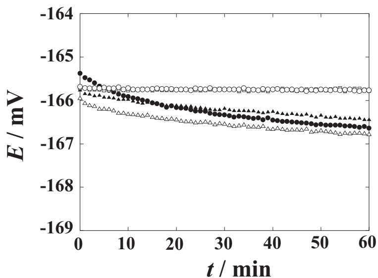
Figure 4.2: Time dependence of E for 1 h at 0.025 \text{ mol kg}^{-1} equimolal phosphate buffer solutions in cell (A) at 15^\circ\text{C} . \circ : 1st measurement, \triangle : 2nd measurement, \square : 3rd measurement, \bullet : 4th measurement, \blacktriangle : 5th measurement.
