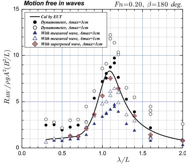
Fig. 2 Added resistance on the blunt modified Wigley model at Fn = 0.2 in the motion-free case.
