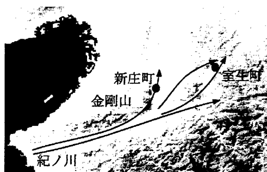
Fig.10 Sketch of dominant stream at 15:00, Sept. 22, 1998 (Typhoon eye locates near Ohmi-Hachiman city near the Lake Biwa)
