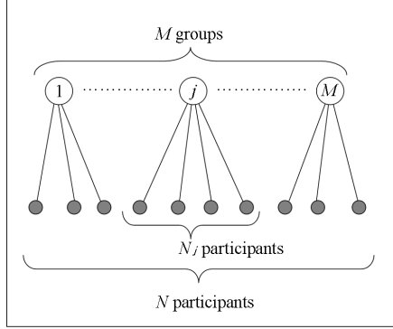
Figure 1: A schematic illustration of a bipartite representation for M groups consisting of N_i ( i = 1, \dots, M ) participants.
