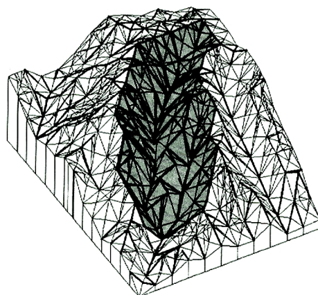
Fig. 12. Three dimensional representation of the upper part of the Ara experimental basin using TIN-DEM data structure.
