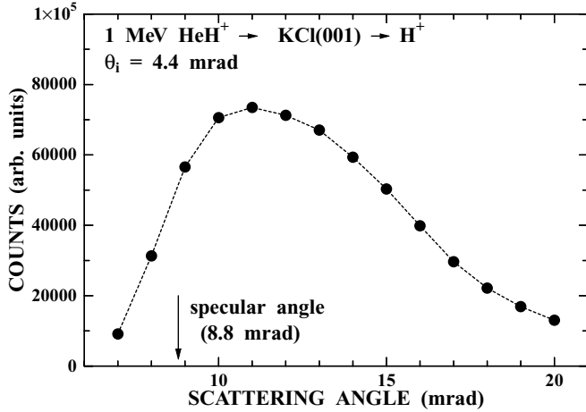
FIG. 3. Scattering angle distributions of protons and He ions observed at \varphi = 0 mrad when 1 MeV \text{HeH}^+ ions are incident on \text{KCl}(001) at \theta_i = 4.4 mrad.
