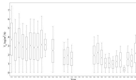
Fig. 7 Temporal frequency distribution of calibrated T_0 parameter ( Eff \geq 0.5 ) for every year (1972 - 2006).
