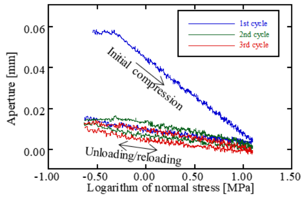
Fig. 6 Aperture evolution during compression tests of Case-1 in specimen G1
