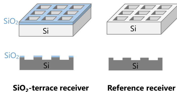
Figure 4. Schematic bird's-eye views and cross-sectional views of the SiO 2 -terrace receiver and the reference Si-only receiver.
