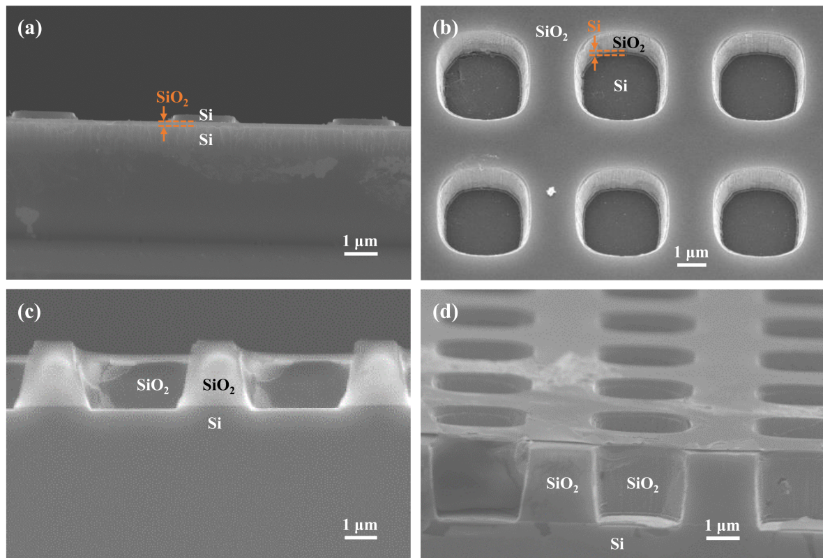
Figure 3. (a) Cross-sectional scanning electron microscope image of the releaser piece, (b) bird's-eye-view and (c) cross-sectional scanning electron microscope images of the receiver piece with an SiO 2 terrace before the submergence process, and (d) bird's-eye-view scanning electron microscope image of the receiver piece with an SiO 2 terrace after the submergence process.
