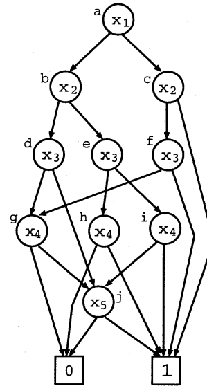
Figure 2: An example of input for Algorithm CheckOTS.
