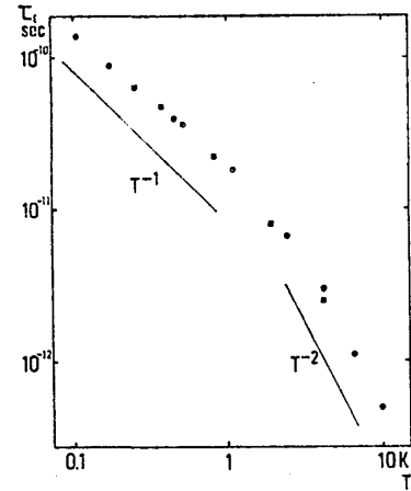
Fig.3 Temperature dependence of inelastic scattering time ( \tau_c ) deduced from the data shown in Fig.1a (●) and 1b (■).
