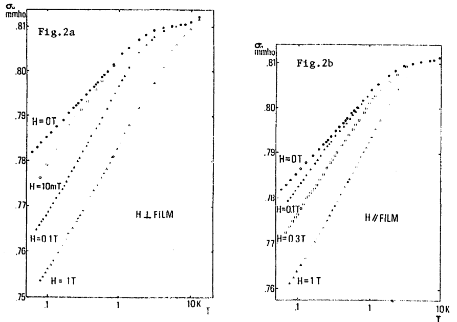
Fig.2 Sheet conductivity of the Bi film vs. temperature in various magnetic field perpendicular (a) and parallel (b) to the film.
