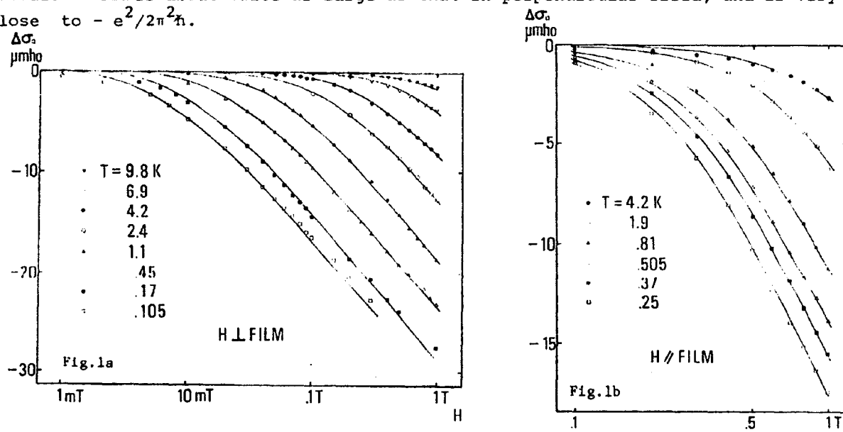
Fig.1 Sheet conductivity of a Bi film vs. magnetic field perpendicular (a) and parallel (b) to the film at various temperatures. Here \Delta\sigma = \sigma(H) - \sigma(0) , and \sigma(0) 's are given in Fig.2. Solid lines are theoretical curves calculated from eq.1 (a) and eq.2 (b) with parameters given in the text.
