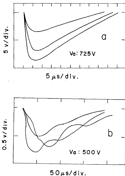
Fig. 1. Outputs signals from the counter. Pulse shapes of the preamplifier outputs when the counter is filled with Q gas and pure He gas are shown by figures a and b, respectively. V_a denotes the voltage applied to the anode wire.
