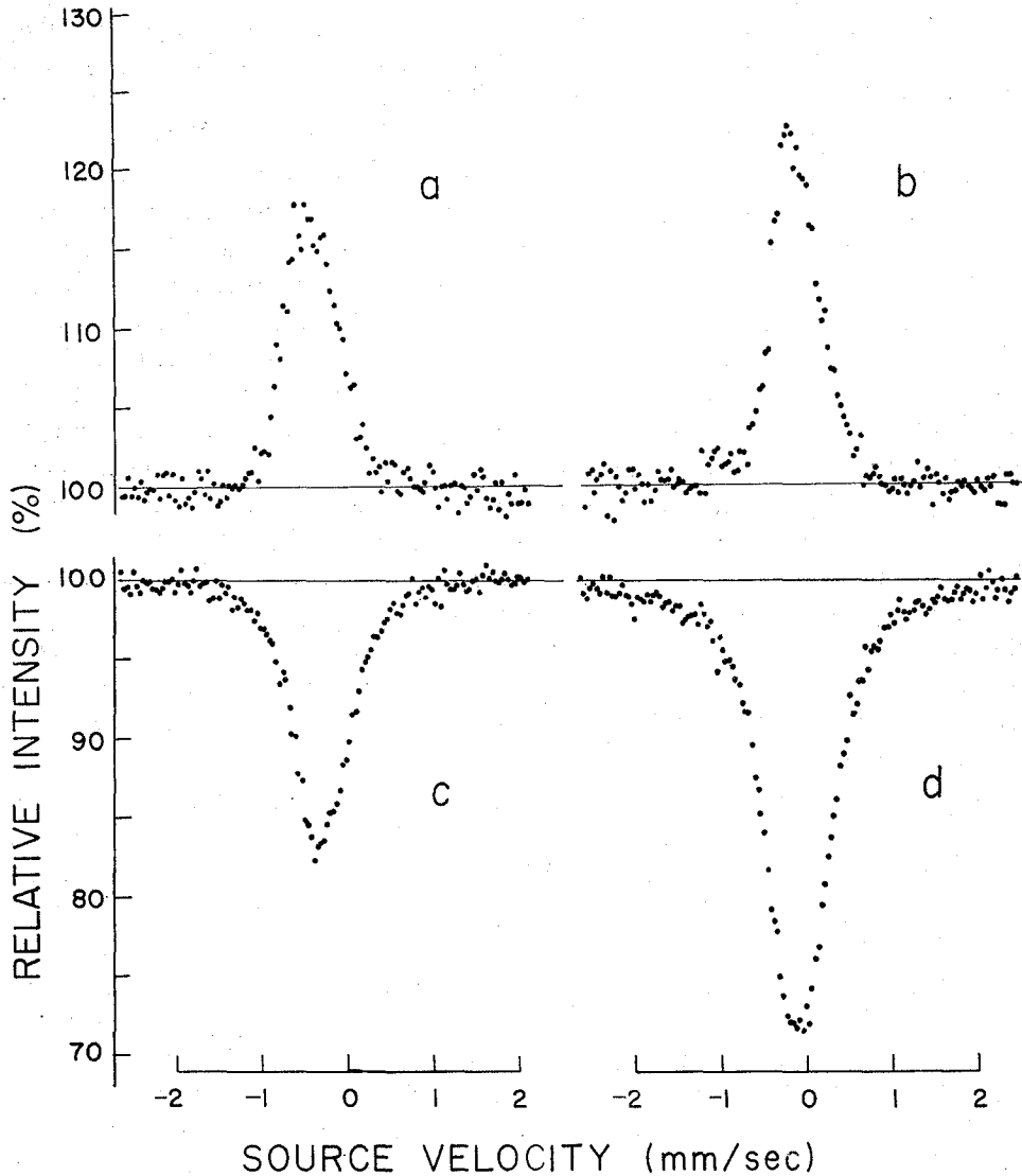
Fig. 2. Mössbauer spectra of Type 310 stainless steel. Spectra a and b are obtained by the present scattering method at 300 K and at 77 K, respectively. For comparison, spectra by the ordinary transmission method are shown by the figures c (at 300 K) and d (at 77 K).
