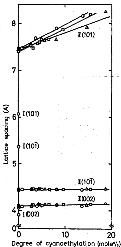
Fig. 6. Lattice spacing vs. degree of cyanoethylation. The values at zero degree of cyanoethylation represent the values for samples immersed in alcoholic 5.4N NaOH. (□) polynosic fiber, (Δ) cuprammonium rayon fiber, (○) cotton fiber.
