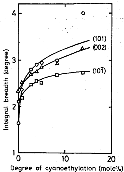
Fig. 9. Integral breadth vs. degree of cyanoethylation for cotton fibers.
