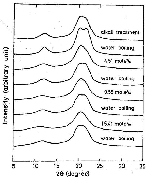
Fig. 10. Effect of boiling in water for 3 hr on the X-ray diffractograms of alkali-acrylonitrile treated polynosic fibers in the presence of alcohol.
