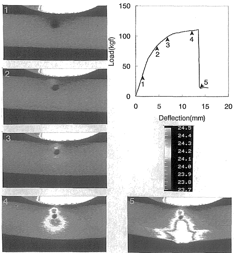
Fig.11. The same as Fig.10, but for specimens with holes in the compressive side.
