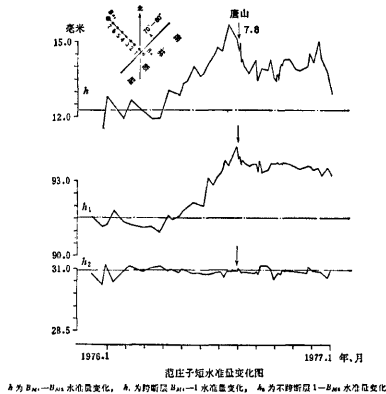
Fig. 5. Crustal movements across an active fault related with the occurrence of the Tangshan earthquake.
