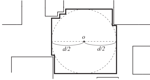
Figure 4.11: Illustration of the minimum enclosing rectilinear polygon of C (represented by thick lines) which is enclosed by R (represented by thin lines)
