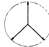
Fig. 8: Three unit horo-normal vectors
