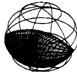
Fig. 10 : Hips ( \kappa_h(0) = 1 of \gamma , a_1 = \text{constant} )
