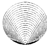
Fig. 3: The axiom of parallel
