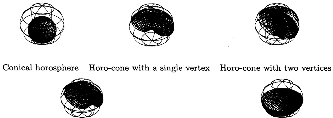
Half cut of horo-cone with a shifted single vertex
