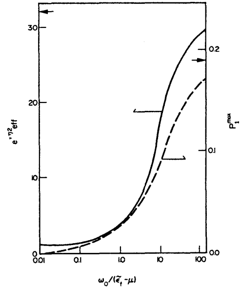
Fig. 2. The inverse of the effective polaron factor, e^{\eta^2_{\text{eff}}} , and the maximum value, P_1^{\text{max}} , in the corrections to P(u) due to the f - d mixing effect, as functions of \omega_0/(\tilde{\epsilon}_f - \mu) . The left scale is for e^{\eta^2_{\text{eff}}} (solid line) and the right scale is for P_1^{\text{max}} (dashed line). The thick arrows denote the limiting values of e^{\eta^2_{\text{eff}}} and P_1^{\text{max}} for \omega_0/(\tilde{\epsilon}_f - \mu) \rightarrow \infty , respectively.
