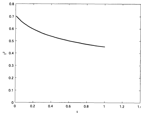
Figure 2. The dissipation property of the scheme (2.4) for (4.1).
