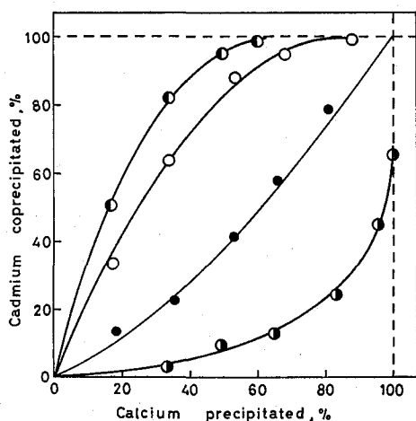
Fig. 3. The coprecipitation of cadmium at various ethylenediamine concentrations.
