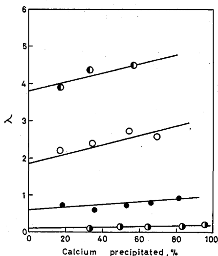
Fig. 4. The apparent distribution coefficient at various ethylenediamine concentrations.
