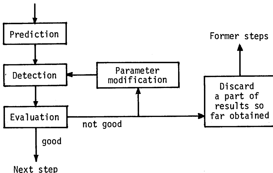
Figure 3-5 Structure of analysis step.
