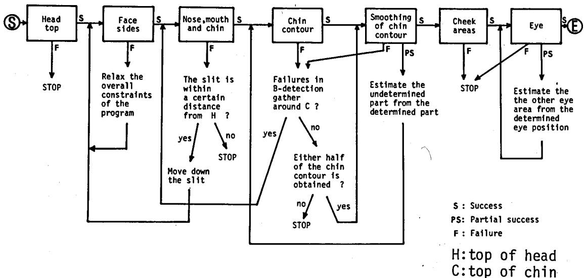
Figure 3-12 General flow of analysis program.
