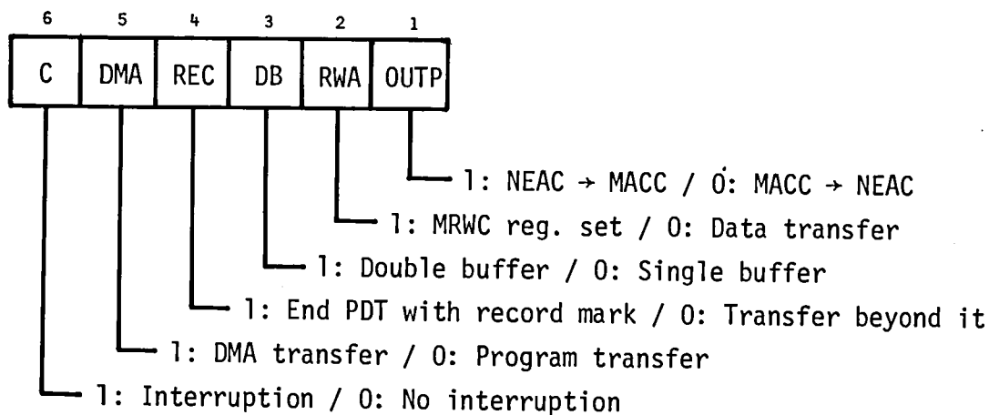
Figure A-4 C_3 of PDT instruction.
