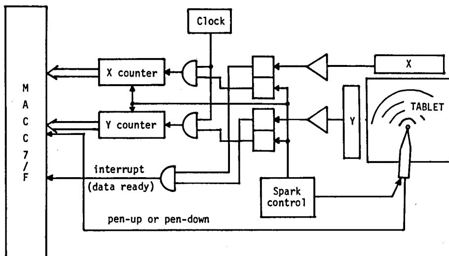
Figure A-9 Diagram of Graf/pen controller.
