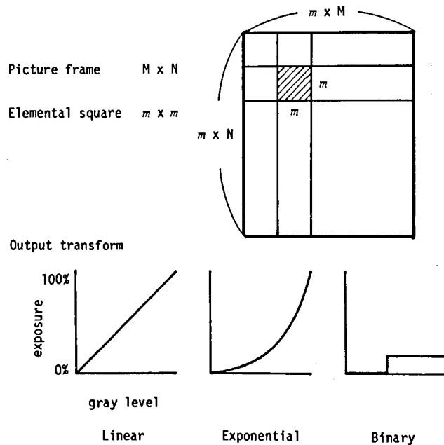
Figure 2-13 Structure of film-recording program.
