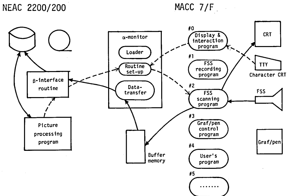
Figure A-12 Software organization of GIRLS.
