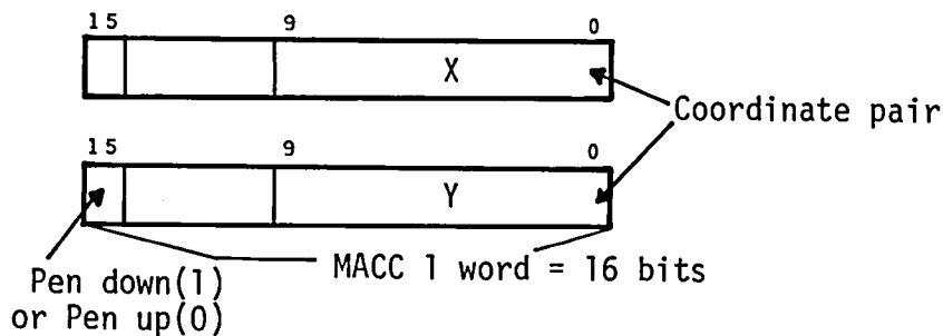
Figure A-10 Data format of Graf/pen.
