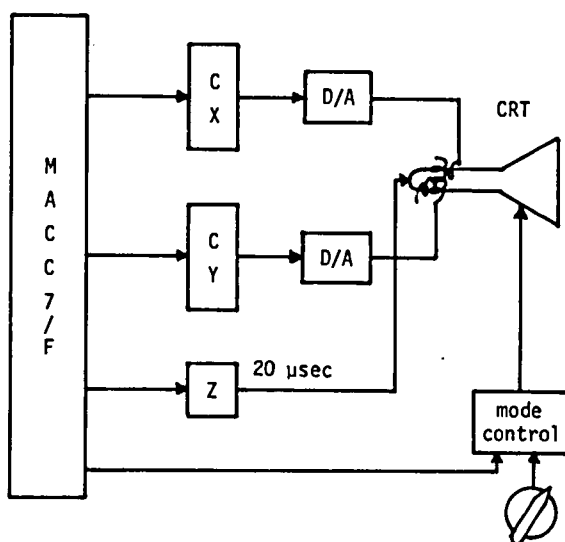
Figure A-11 Diagram of CRT controller.
