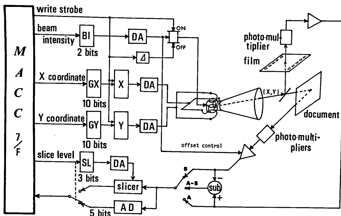
Figure A-6 Functional diagram of FSS controller.
