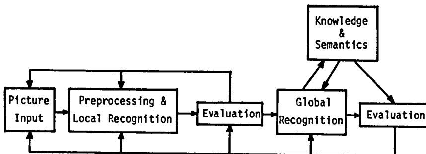
Figure 2-1 Advanced picture processing scheme.
