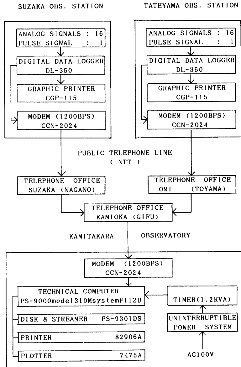
Fig. 5. Block diagram of the system for data collecting, telemetering and data processing.
